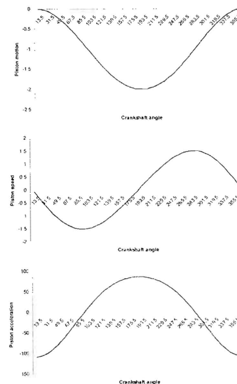
Figure 8: Simulation of single cylinder motor's kinematics
