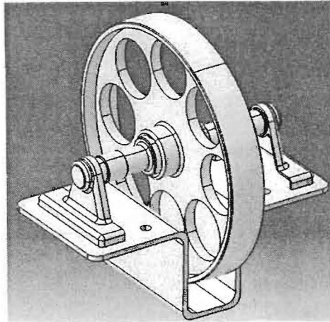
Figure 6: Assembly simulation
