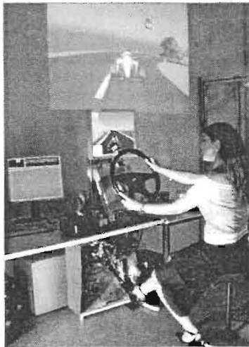
Figure 13: MechatronicCarLab with force-reflecting steering input devices (steering wheel, joystick) and force-reflecting accelerator pedal, real-time vehicle dynamics simulation and visualization
