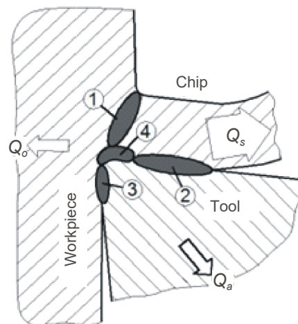
Figure 1. Heat sources and distribution of heat during cutting process [16]; Q_s – the heat transferred from heat sources to the chip, Q_a – the heat transferred from heat sources to the tool, Q_o – the heat transferred from heat sources to the workpiece
