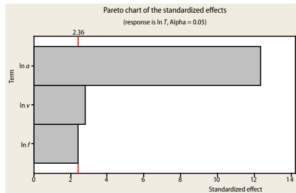
Figure 6. Effects of end milling parameters on temperature
