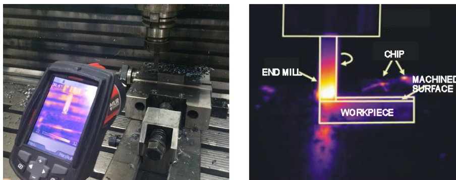
Figure 4. Infrared camera position and thermogram
