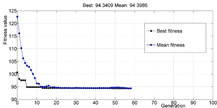
Figure 7. The GA optimization process
