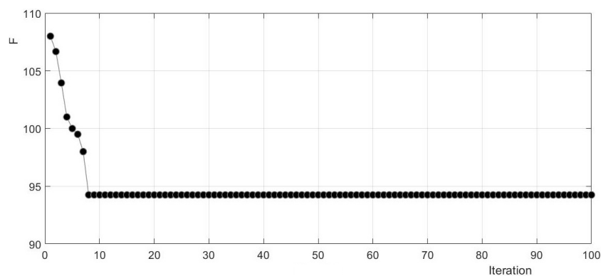
Figure 8. The PSO optimization process
