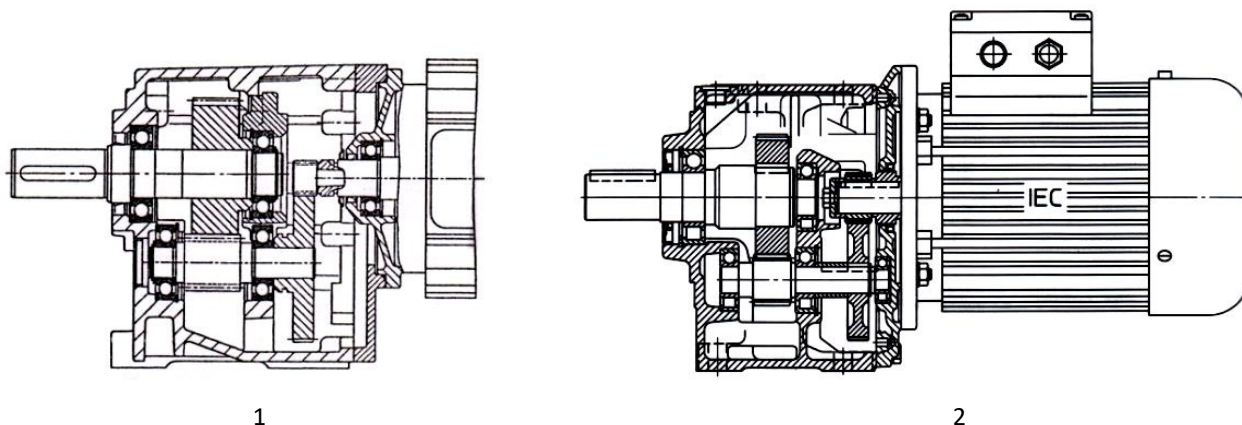
Fig.2. Gearmotor with special reducer motor Lenze (1) and gearmotor with standard electric motor ROSSI (2) [7,8]
