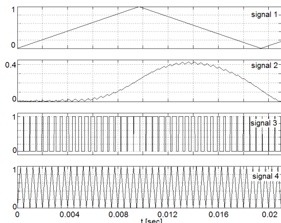
Fig. 2. Waveforms of the characteristic control signal of the switching power converter
