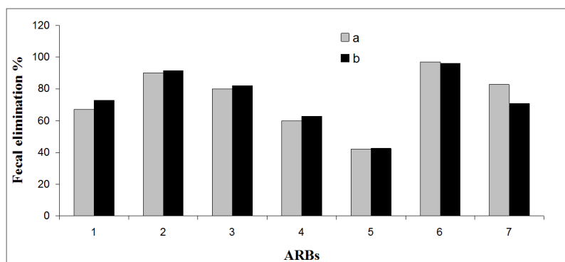
Fig. 1. The relationship between ARBs fecal elimination data from literature (a) and predicted (b) fecal elimination data (using Clog P , and log S values) ( R^2 = 0.909 ). ARBs - Angiotensin II receptor antagonists; 1 - candesartan; 2 - eprosartan; 3 - irbesartan; 4 - losartan; 5 - olmesartan; 6 - telmisartan; 7 - valsartan.
