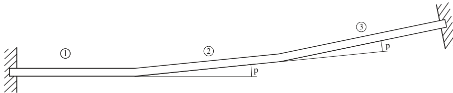
FIGURE 6. The initial position of the frame structure with clamped ends in the case of veering, ( p = 0.1 )
