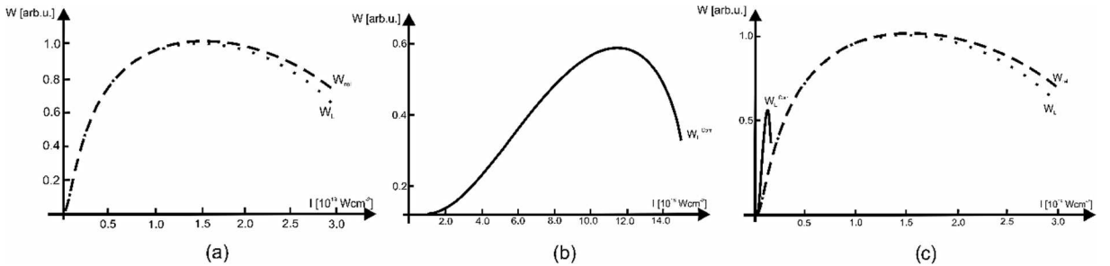
Figure 1. Comparative review of the transition rate of: a) W_{rel} and W_L (the dotted curve represents calculations by the formulas of (DELIBAŠIĆ et al. , 2018)), b) W_L^{Corr} and c) W_L^{Corr} , W_L and W_{rel} . The laser intensity is within the range: I = 0.5 \times 10^{19} - 3 \times 10^{19} \text{ Wcm}^{-2} .
