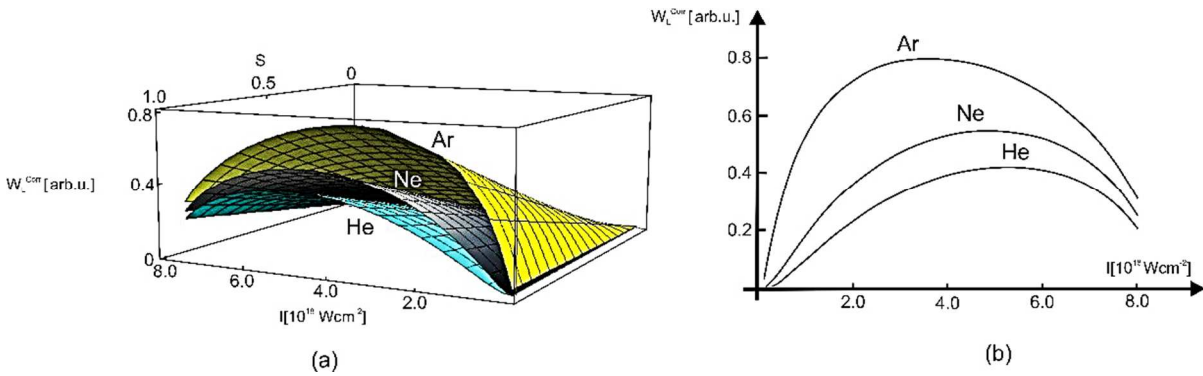
Figure 2. a) 3D graph for W_L^{Corr} as a function of the field intensity, I and the stabilization factor S , for noble, single ionized, Z = 1 , Ar , Ne and He atoms. The stabilization factor is within the range 0 \leq S \leq 1 , b) 2D graph, W_L^{Corr} as a function of the field intensity, I . For both graphs intensity varies within the range I = 1 \times 10^{18} - 8 \times 10^{18} \text{ Wcm}^{-2} .
