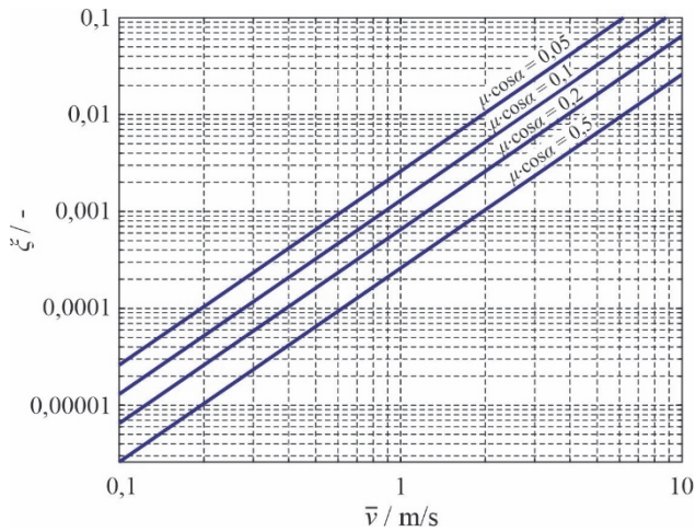
Figure 6 Change of coefficient \xi as the function of sliding velocity \bar{v}
