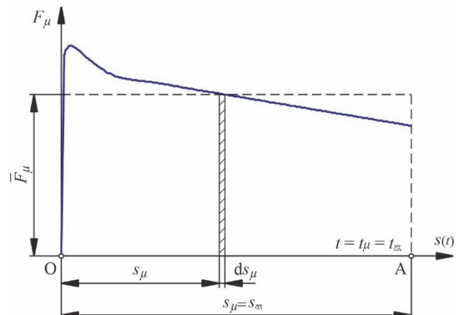
Figure 2 Work of frictional force along the inclined plane
