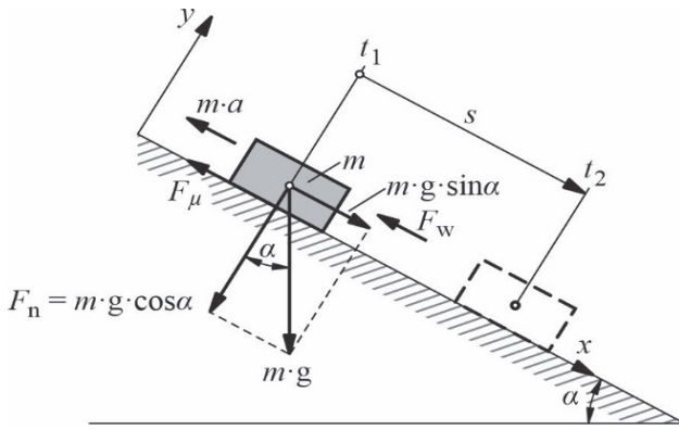
Figure 1 Sliding along an inclined plane
