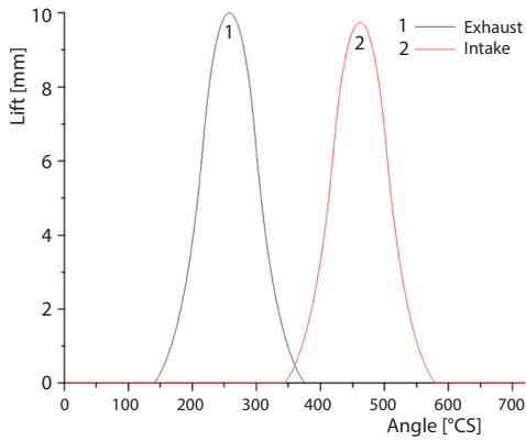
Figure 3. Valve lift profile
