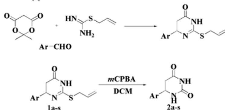
Scheme 1. General outline of the synthesis of DHUs [41].
