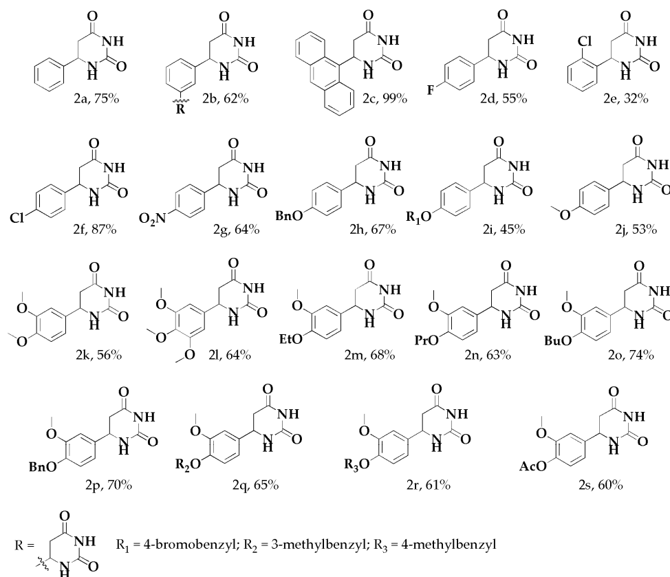
Figure 2. Structures and isolated yields of the DHUs.
