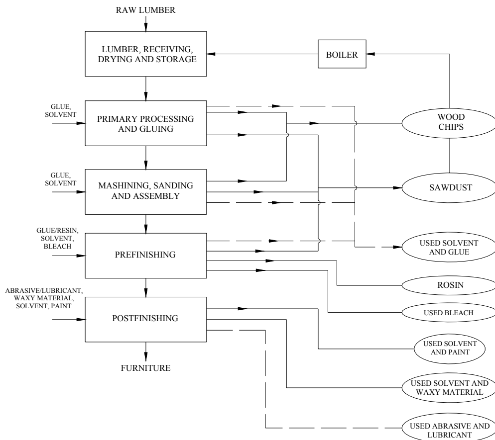
Fig. 1. Flow diagram of the manufacturing processes and materials in a company of this industry
