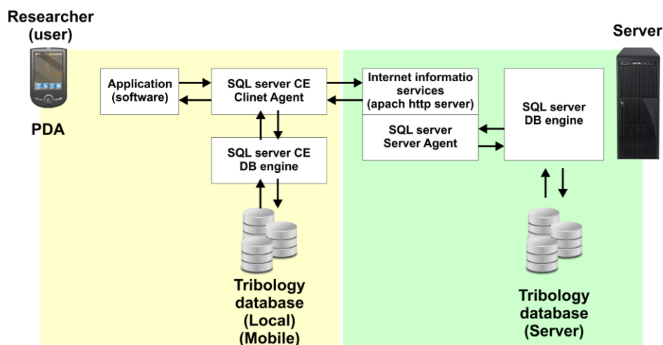
Fig. 11. Replication architecture.
