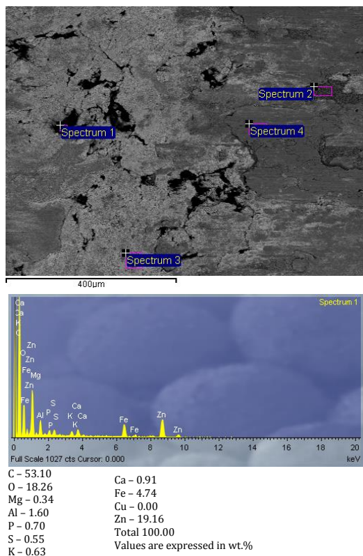
Fig. 9. SEM and EDS wear track analysis of ZA-27 composite reinforced with 1 vol. % of graphite [9].
