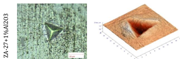
Fig. 6. Indentation imprints analysed by optical and AFM microscopy [10].
