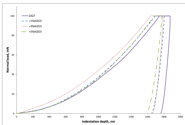
Fig. 5. Nanoindentation curves for ZA-27 alloy and tested nanocomposites reinforced with 1, 3 and 5 vol. % of Al_2O_3 [9].
