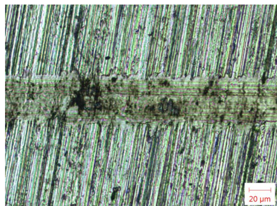
Fig. 8. Optical microscopy of wear tracks for ZA-27 nanocomposite reinforced with 1 vol. % Al_2O_3 , obtained under 200 mN normal load and 2 mm/s sliding distance [10].
