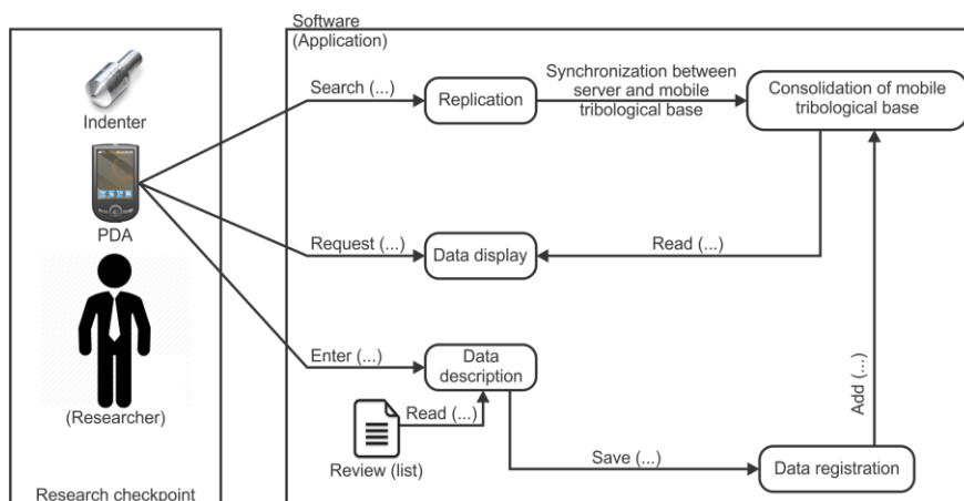
Fig. 10. UML application model of tribology mobile database use.
