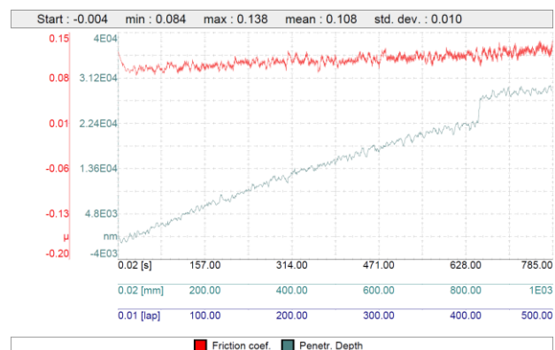
Fig. 7. Friction force and penetration depth dependence on time/sliding distance/laps for ZA-27 nanocomposite reinforced with 1 vol. % Al_2O_3 , obtained under 200 mN normal load and 2 mm/s sliding distance [9].
