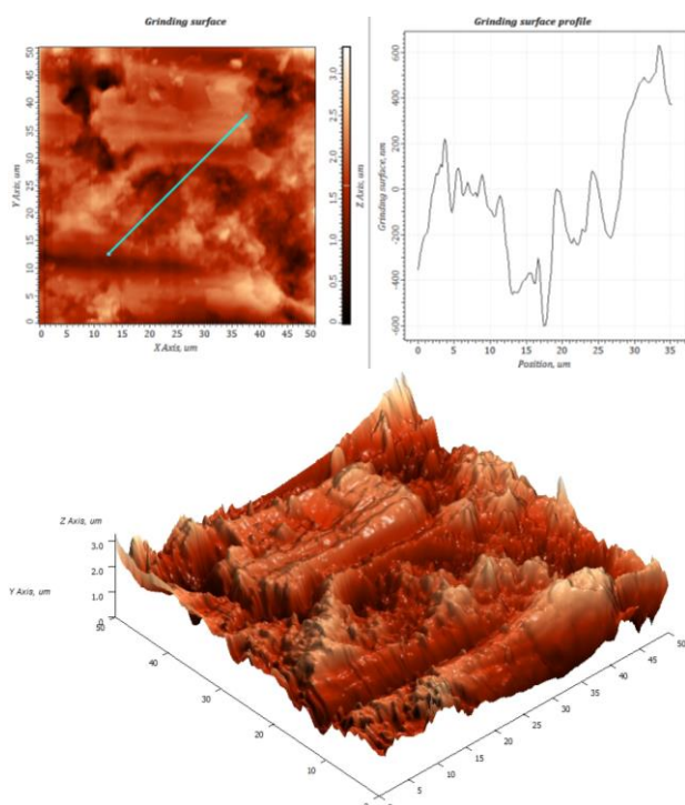
Fig. 4. 3D topography and roughness profile of grinding surface of the lithium disilicate glass ceramic [8].
