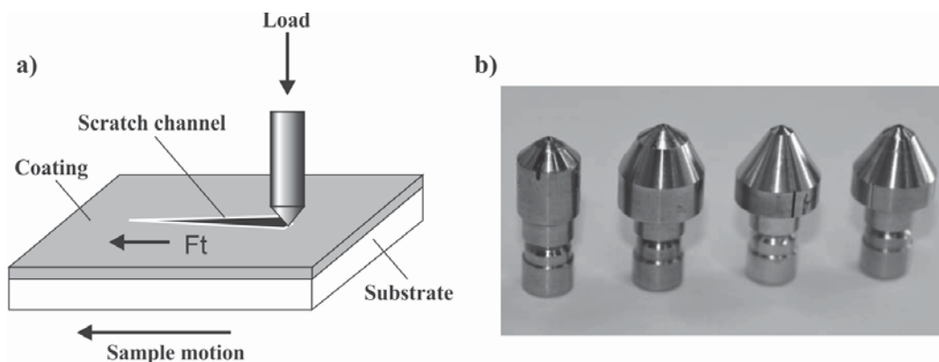
Figure 1: a) Scratch test; b) Rockwell diamond stylus indenter /18/
