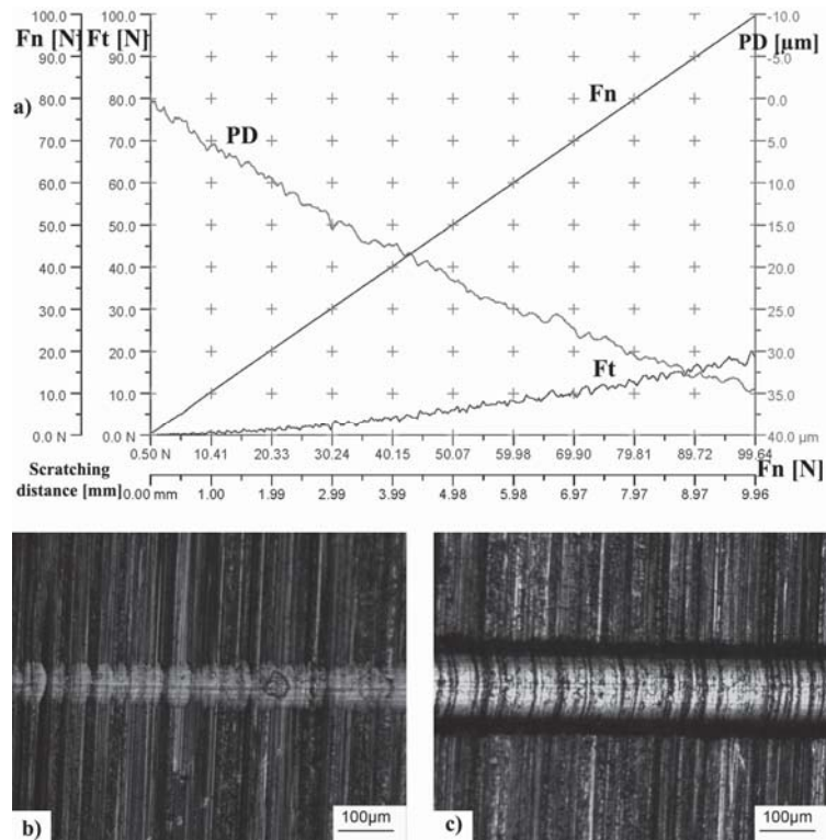
Figure 4: a) Diagram of the friction force, normal force and penetration depth during scratch testing the chrome coating, R_a = 0.4 \mu\text{m} ; Optical micrographs of the scratching scar at critical loads: b) L_{c1} ; c) L_{c2}
