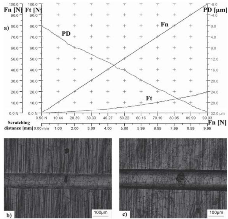
Figure 2: a) Diagram of the friction force, normal force and penetration depth during scratch testing of the chrome coating, R_a = 0.01 \mu\text{m} ; Optical micrographs of the scratching scar at critical loads: b) L_{c1} ; c) L_{c2}
