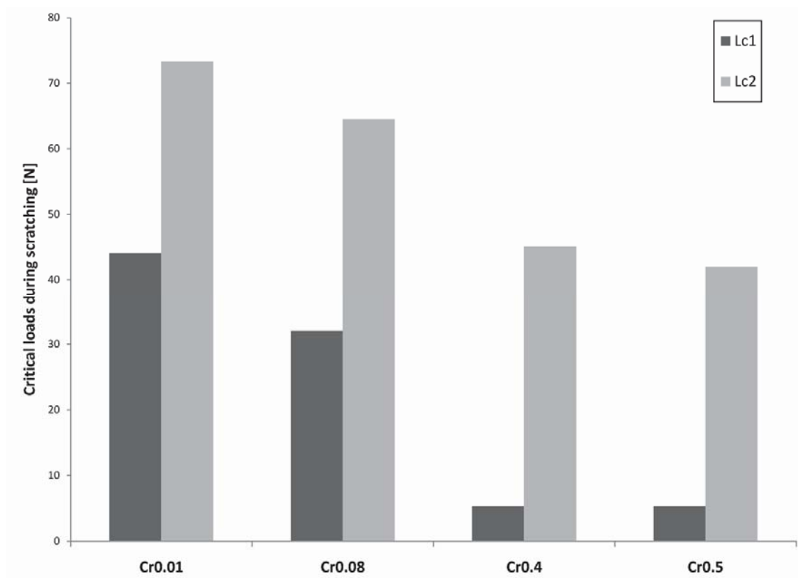
Figure 7: Influence of the coating surface roughness on coating adhesion: critical loads during the scratch test for different coating surface roughness
