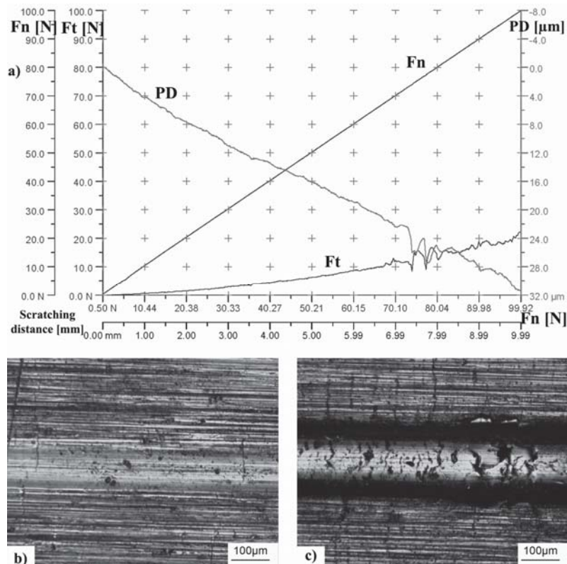
Figure 3: a) Diagram of the friction force, normal force and penetration depth during scratch testing the chrome coating, R_a = 0.08 \mu\text{m} ; Optical micrographs of the scratching scar at critical loads: b) L_{c1} ; c) L_{c2}
