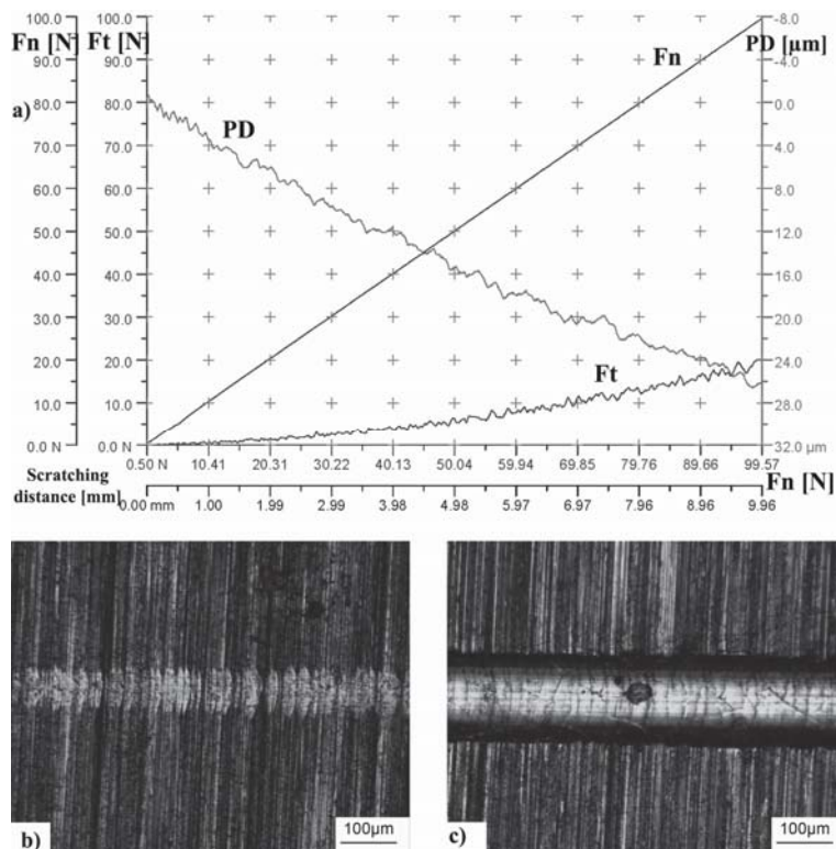
Figure 5: a) Diagram of the friction force, normal force and penetration depth during scratch testing the chrome coating, R_a = 0.5 \mu\text{m} ; Optical micrographs of the scratching scar at critical loads: b) L_{c1} ; c) L_{c2}
