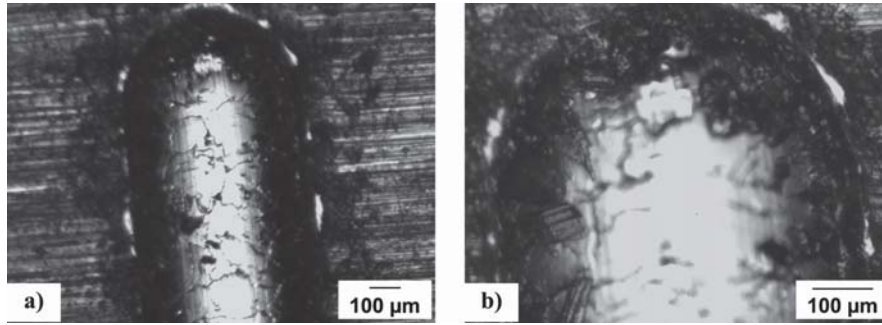
Figure 6: Crack pattern produced after scratching, on the chrome coating of R_a = 0.5 \mu\text{m} surface roughness
