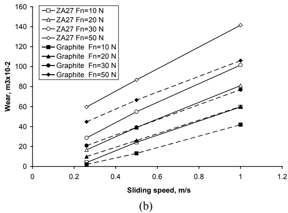
Fig. 18. Wear volume vs. sliding speed: (a) lubricated sliding, (b) dry sliding
