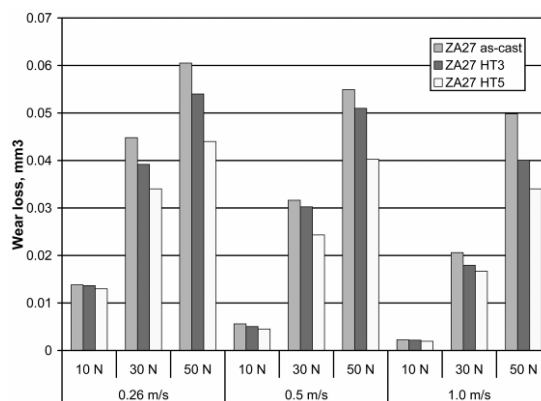
Fig. 10. Wear volume loss of tested alloys comparison
