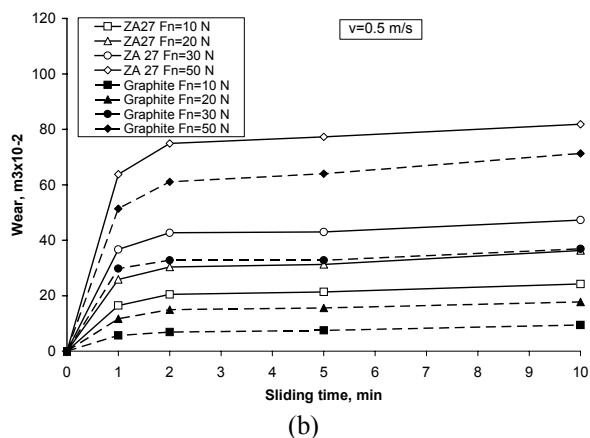
Fig. 16. Wear curves of tested samples in conditions of lubricated (a) and dry sliding conditions (b)
