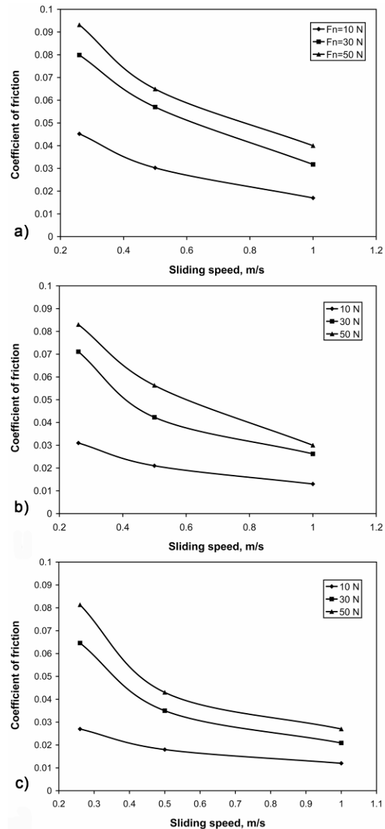
Fig. 6. Friction coefficient vs. sliding speed for different applied loads: (a) ZA27 as-cast, (b) ZA27 HT3, (c) ZA27 HT5 (lubricated tests)
