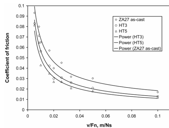
Fig. 7. Friction coefficient of tested alloys vs. speed-to-load ratio (lubricated tests)
