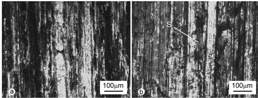
Fig. 21. Worn surfaces in conditions of dry sliding with 50 N of applied load and 1.0 m/s of sliding speed: (a) ZA-27, (b) Graphite particles reinforced ZA-27 alloy composite
