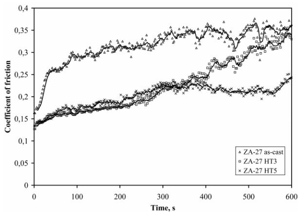
Fig. 12. Coefficient of friction vs. sliding time curves for ZA-27 alloy in as-cast and heat-treated conditions (applied load 15 N, sliding speed 0.26 m/s) (dry sliding)
