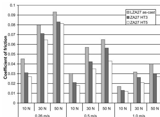
Fig. 9. Friction coefficient of tested alloys comparison
