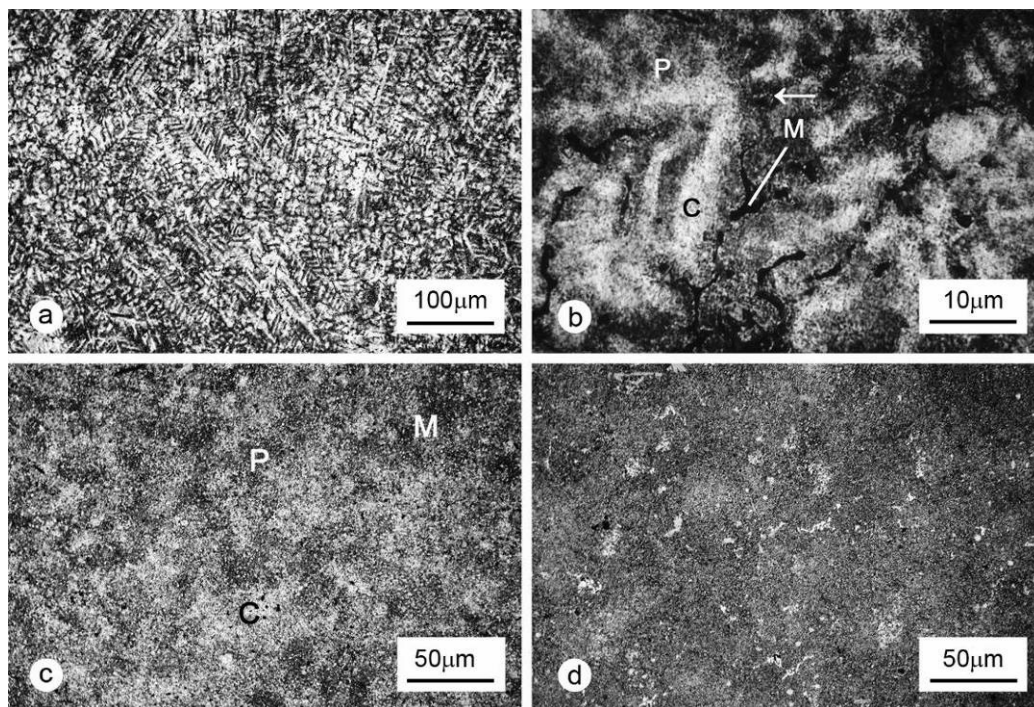
Fig. 2. Microstructure of the alloy: (a and b) as-cast, (c) heat-treated with 3 h and (d) 5 h of solutionizing (C– \alpha dendrite core, P – \alpha+\eta dendrites’ periphery, M – \eta interdendritic phase)
