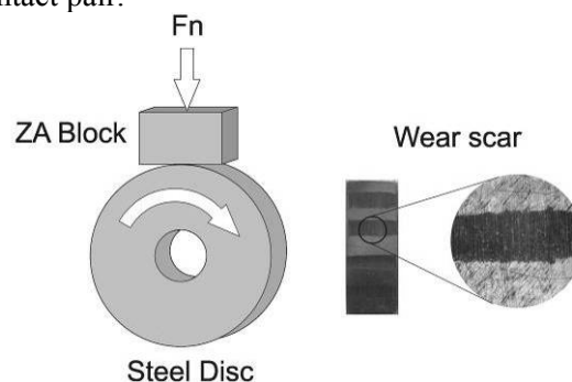
Fig. 1. The scheme of contact pair geometry
