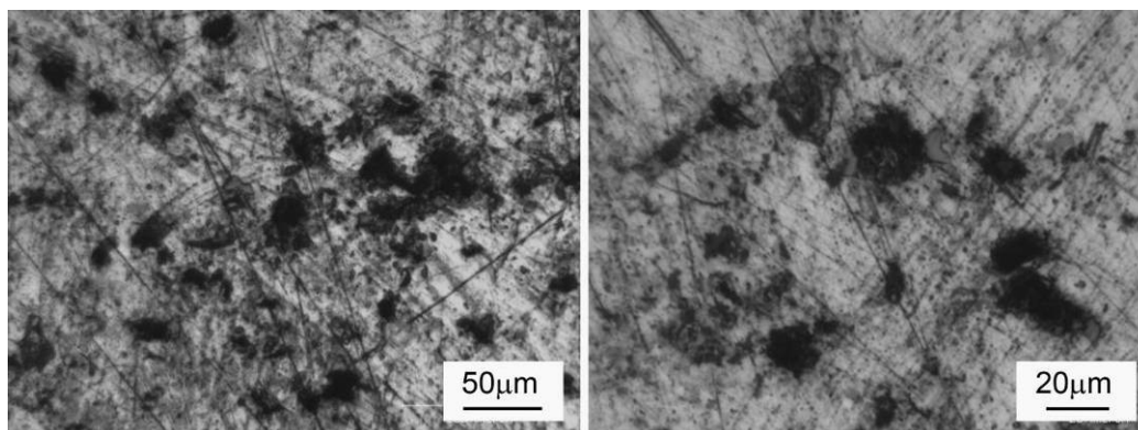
Fig. 3. Optical micrograph of graphite particles reinforced ZA-27 alloy composite materials (polished surface)
