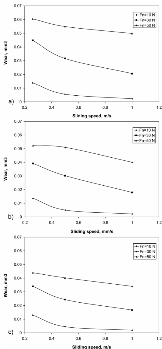
Fig. 8. Wear loss of tested alloys vs. sliding speed for different applied loads: (a) ZA27 as-cast, (b) ZA27 HT3, (c) ZA27 HT5
