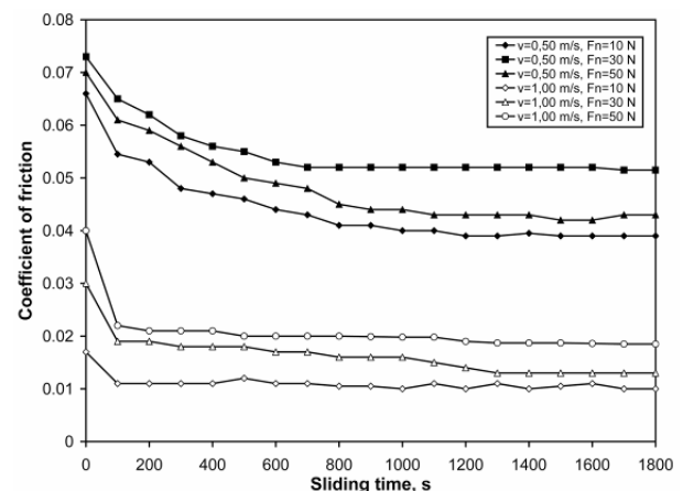
Fig. 5. Friction coefficient variation of ZA27 HT5 during sliding time at different specific loads and sliding speeds (lubricated tests)
