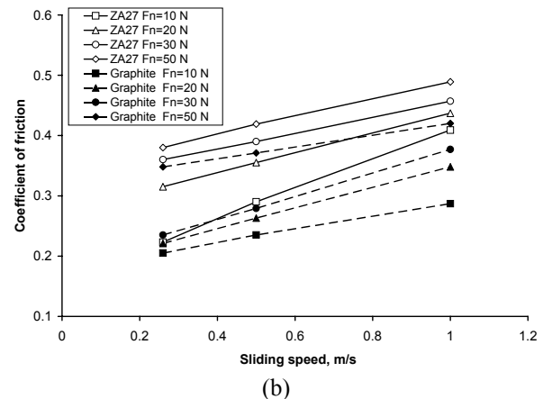
Fig. 20. Coefficient of friction vs. sliding speed: (a) lubricated sliding, (b) dry sliding
