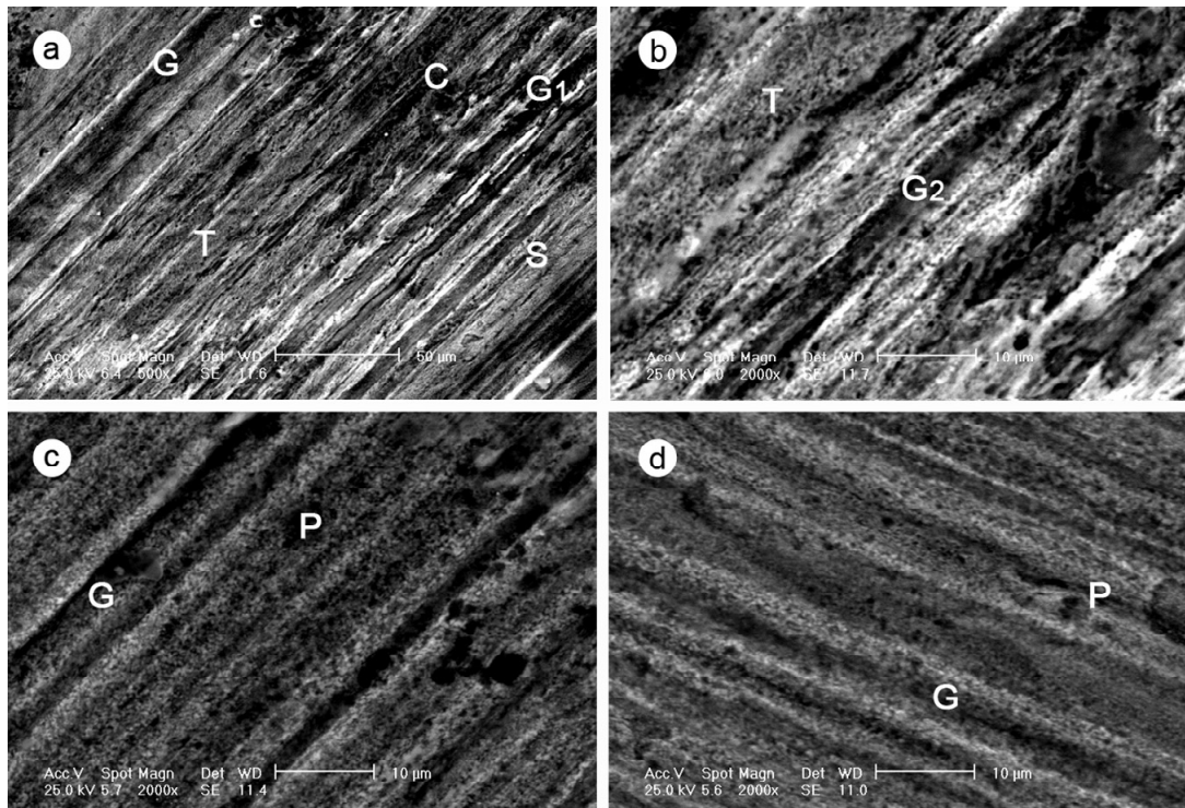
Fig. 11. Wear surface of the alloys in lubricated sliding for 50 N of applied load and 0.26 m/s of sliding speed in conditions of lubricated sliding: a) ZA27 as-cast alloy, (b) ZA27 HT3 alloy, (c) ZA27 HT5 alloy
