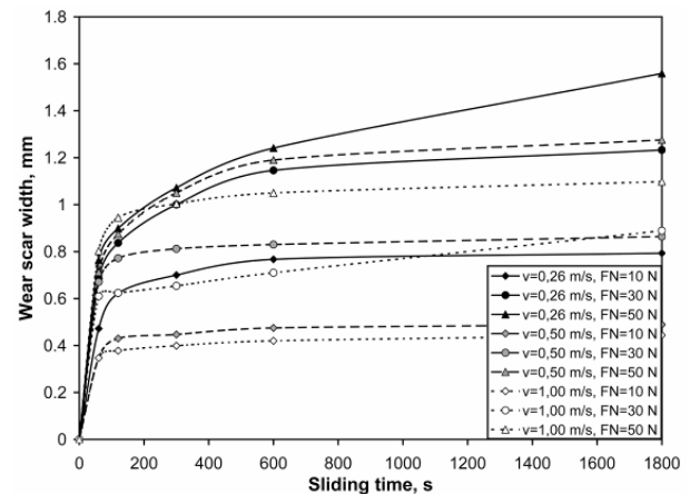
Fig. 4. Wear curves of ZA27 HT5 alloy at different specific loads and sliding speeds (lubricated tests)
