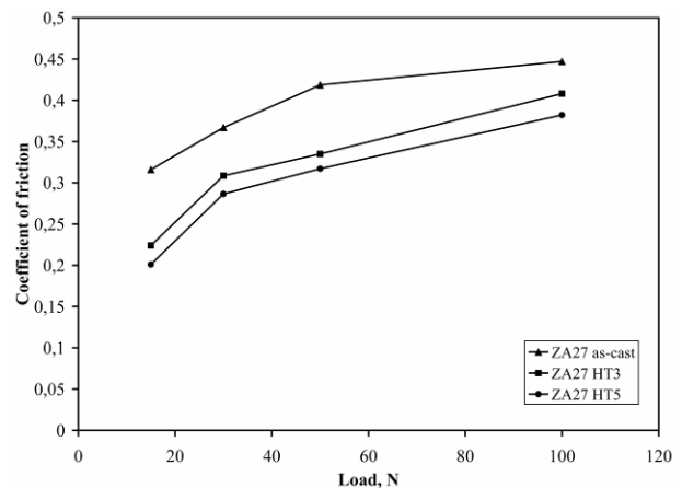
Fig. 13. Coefficient of friction vs. applied load for ZA-27 alloy in as-cast and heat-treated conditions (dry sliding)
