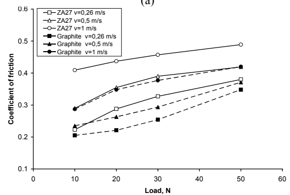
Fig. 19. Coefficient of friction vs. applied load: (a) lubricated sliding, (b) dry sliding
