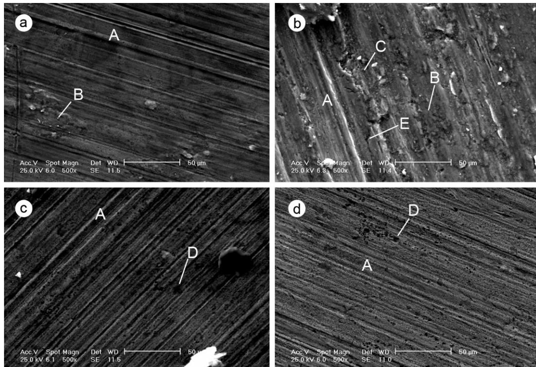
Fig. 15. Wear surfaces of the ZA-27 alloy in as as-cast conditions for applied load of 15 N (a) and 50 N (b) and after heat treatment for applied load of 50 N: (c) ZA-27 HT3 and (d) ZA-27HT5 (A - ploughing grooves B- smeared material, C -spalls , D – pits , E - surface cracks) (dry sliding)
