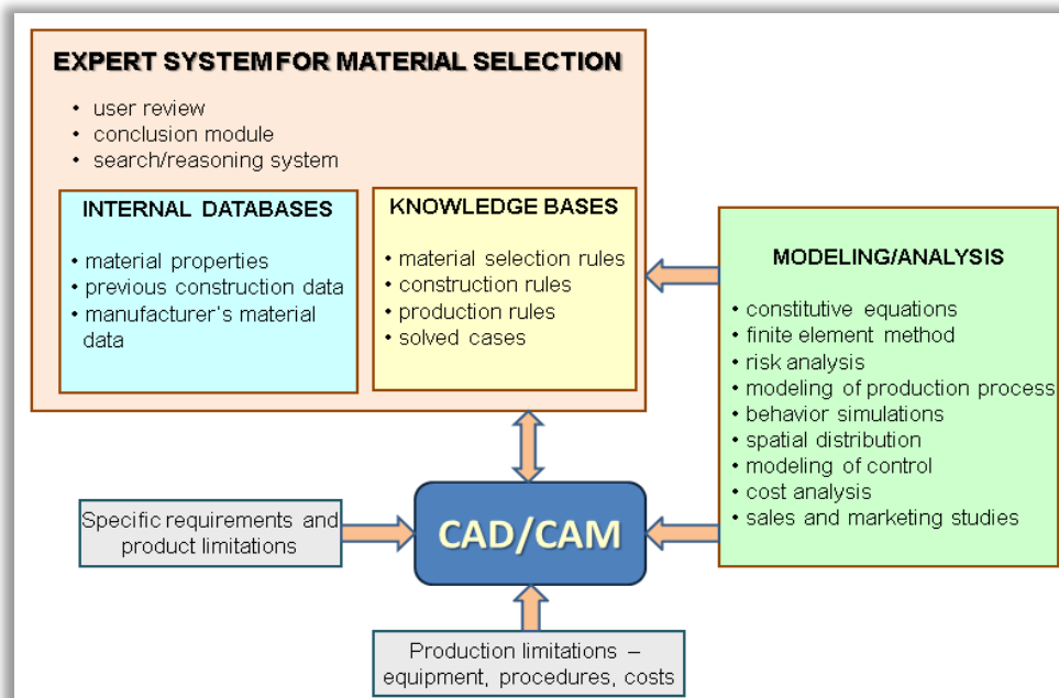
Figure 3. The conceptual scheme of the structure and functioning of the system's expert system [6]
