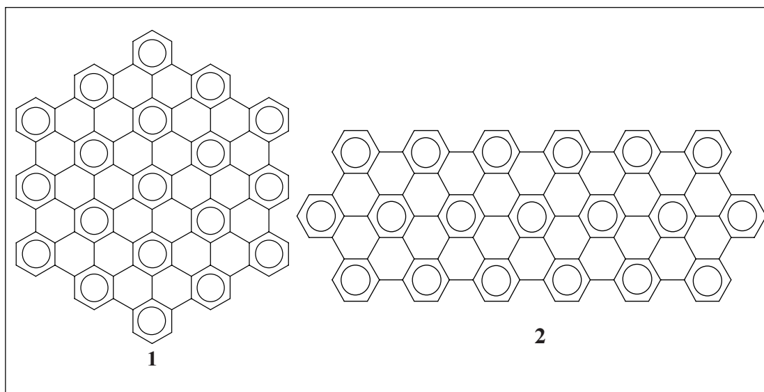
Figure 1. Two large graphenes, both with 114 carbon atoms: 1 = C_{114}H_{30} ; 2 = C_{114}H_{34} .
