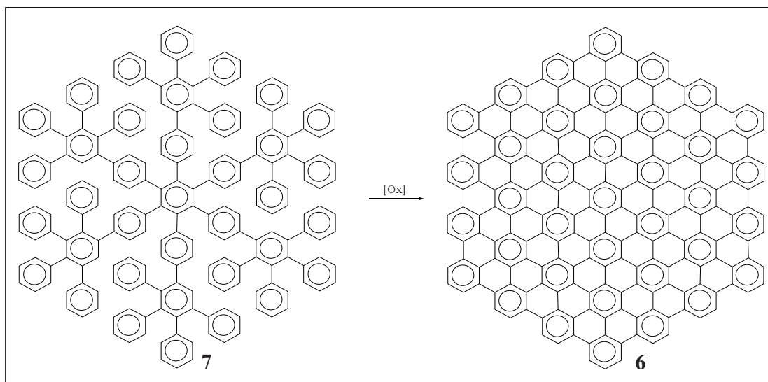
Figure 4b. The second phase of synthesis of graphene: By a single-step oxidation of the polyphenyl 7, graphene 6 is gained in high yield. \text{FeCl}_3 is used as the oxidizing agent.
