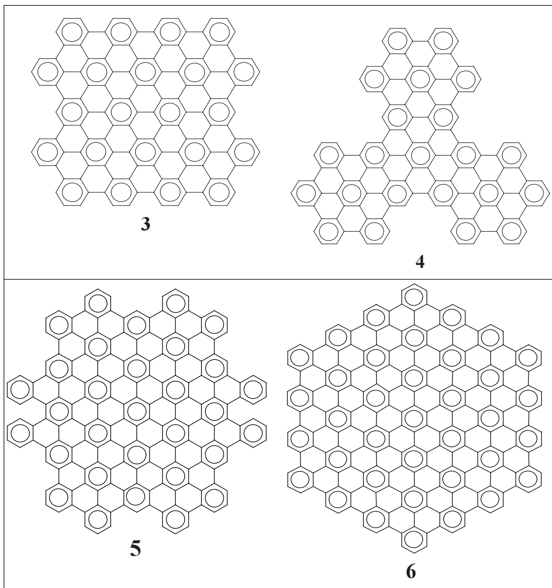
Figure 2 (top). Two still bigger graphenes, both with 132 carbon atoms: 3 = C_{132}H_{34} , 4 = C_{132}H_{42} . Figure 3 (bottom). The two biggest graphenes synthesized so far: 5 = C_{186}H_{46} , 6 = C_{222}H_{40} . It is worth noting that compound 6 contains only 1.48% hydrogen, whereas the rest is carbon.
