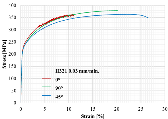
Fig. 2. Stress–strain curves for different direction of rolling.
