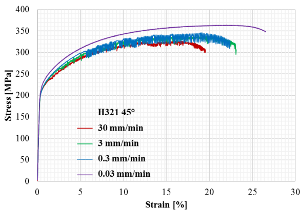
Fig. 1. Stress–strain curves for different strain-rates.
