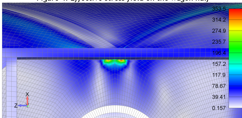
Figure 5. Effective stress field on the welding of the first tank and longitudinal girder
