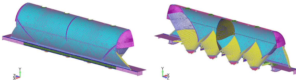
Figure 3. FEM model of wagon half
