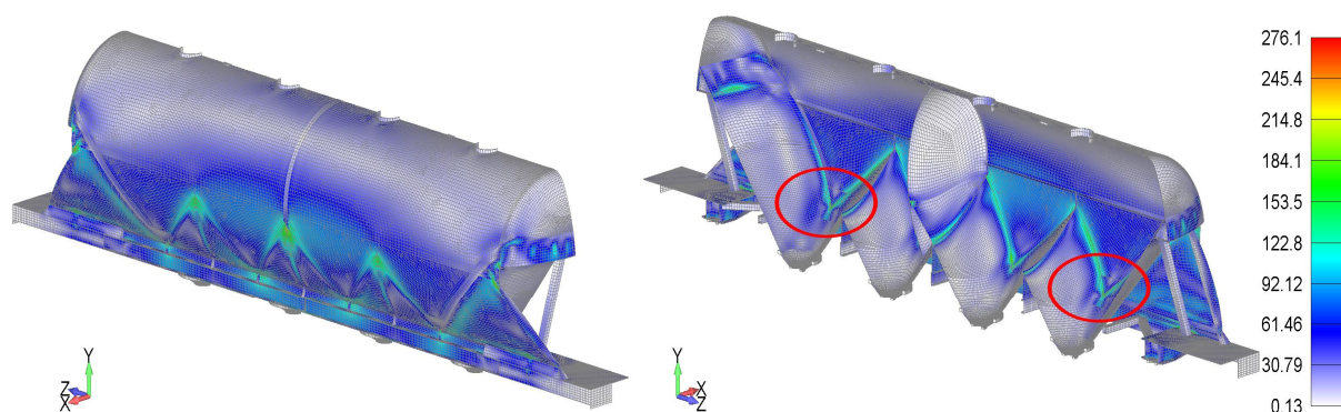
Figure 7. Effective stress field on the reconstructed model
