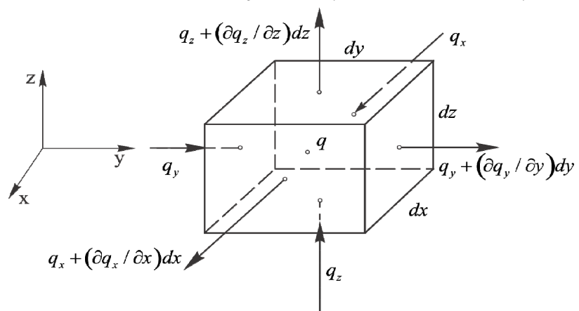
Figure 1. Elementary volume dV with heat flux components
