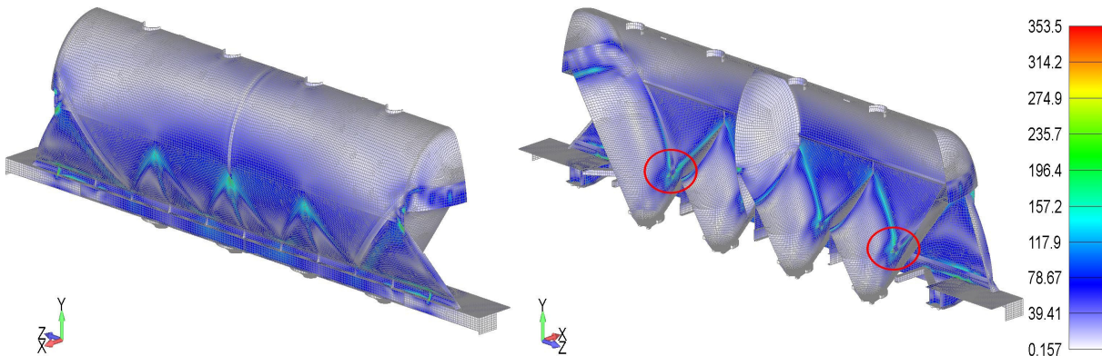
Figure 4. Effective stress field on the wagon half
