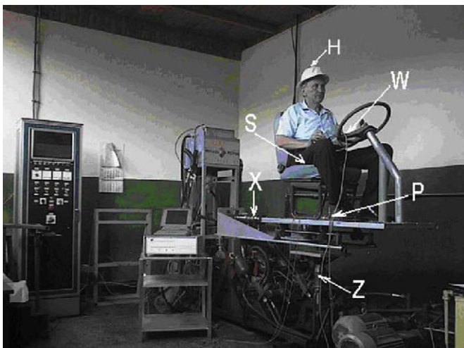
Fig. 1. Measurement equipment.
