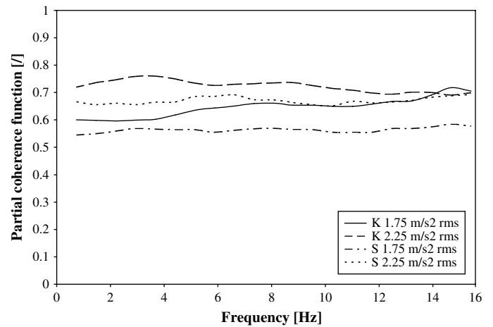
Fig. 10. Partial coherence function \gamma_{4y,3}^2 in vertical direction.
