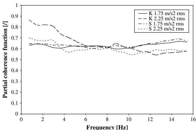
Fig. 9. Partial coherence function \gamma_{3y,2}^2 in vertical direction.
