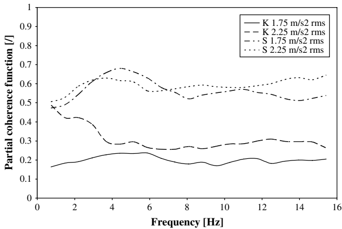
Fig. 8. Partial coherence function \gamma_{6y,5}^2 in fore and aft direction.
