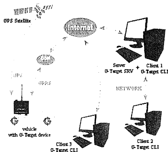
Figure 2: G-Target AVL system
