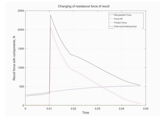
Figure 3. Components of the recoil resistance force and the total recoil resistance force [6]
