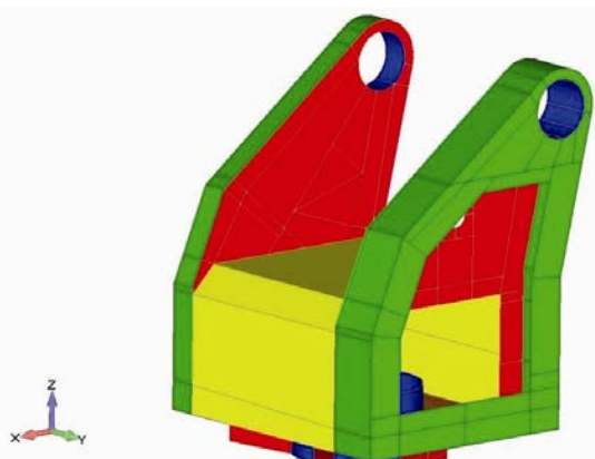
Figure 4. Display of the model of the middle surfaces of the structure of the upper carriage in the software package FEMAP.
