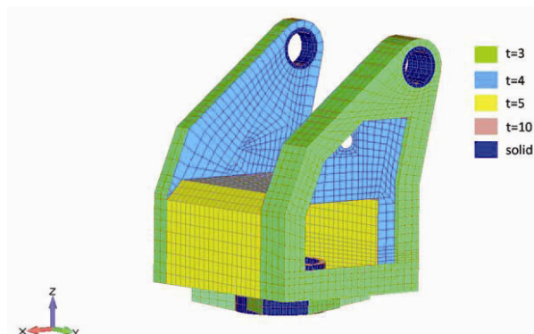
Figure 5. MKE upper carriage construction model
