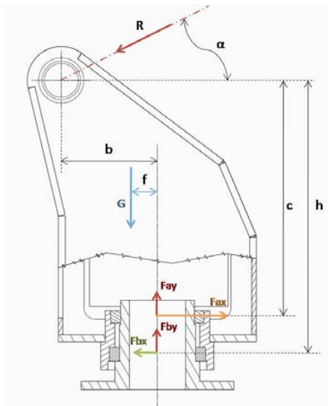
Figure 1. Schematic representation of the forces acting on the upper carriage during firing
