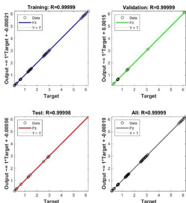
Figure 4. Regression of optimal architecture
