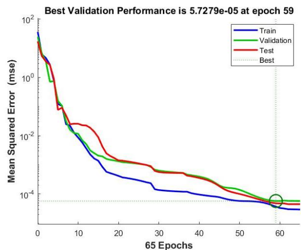
Figure 3. Performance of optimal architecture
