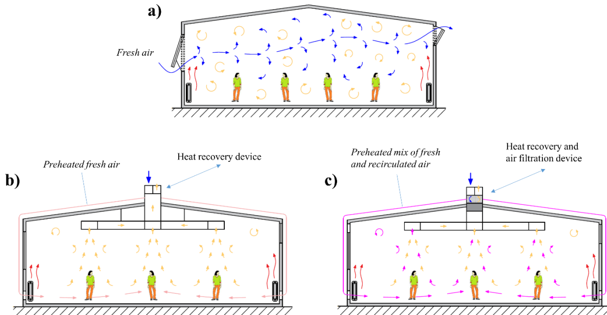
Figure 2. PWH ventilation scenarios, a) NV, b) FBV, c) FBV-FAR
