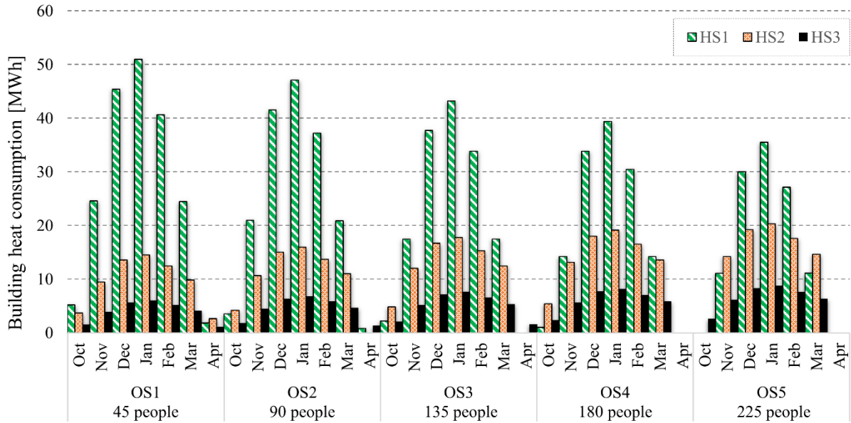
Figure 4. PHW heat demand for various simulation scenarios
