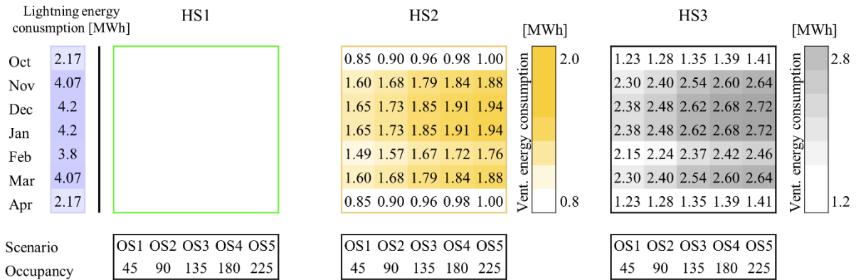
Figure 5. Monthly PWH HVAC energy consumption
