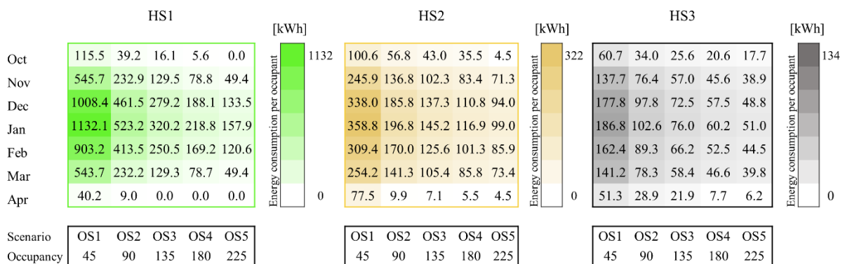
Figure 7. Monthly indicators of PHW energy consumption (kWh/occupant)
