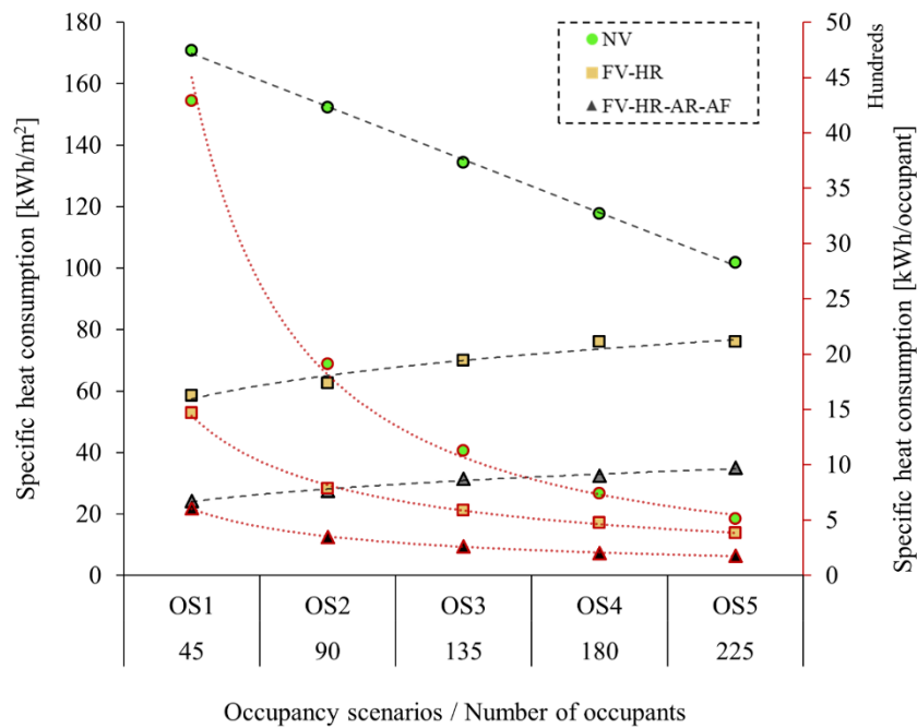
Figure 6. Seasonal indicators of PWH energy consumption
