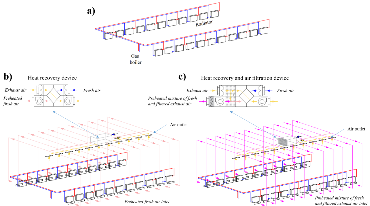
Figure 3. PHW heating scenarios, a) CHR, b) CHR-HR, c) CHR-HR-AR
