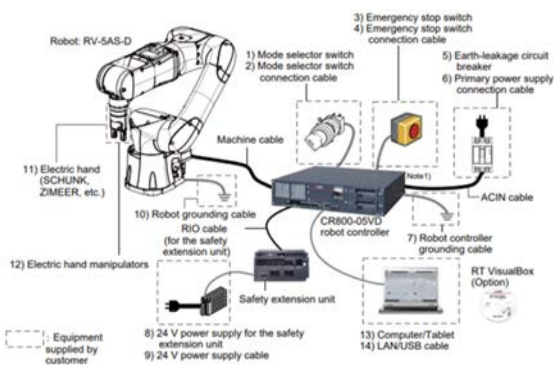
Figure 2. Basic components necessary for collaborative robot operation
