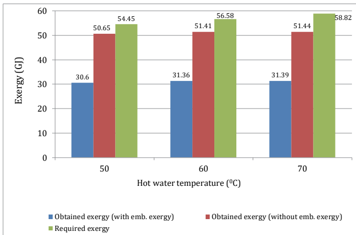
Fig. 3 Required and obtained exergy for building with defferent hot water temperature
