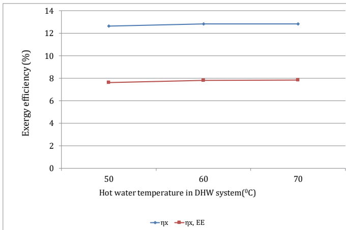
Fig. 2 Exergy efficiency for building with defferent hot water temperature
