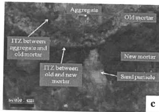
Figure 1. Sectional view of RCA [18]
