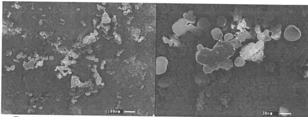
Figure 5. Scanning electron micrograph of recycled aggregate grain (w/c = 0.45, fraction 12/16 mm) after biodeposition treatment [25]
