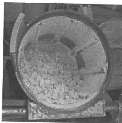
Figure 2. The mill drum [2]
