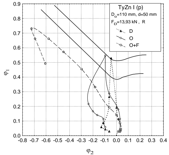
Figure 11. Strain distributions in sheet metal plane (CBF-R)
