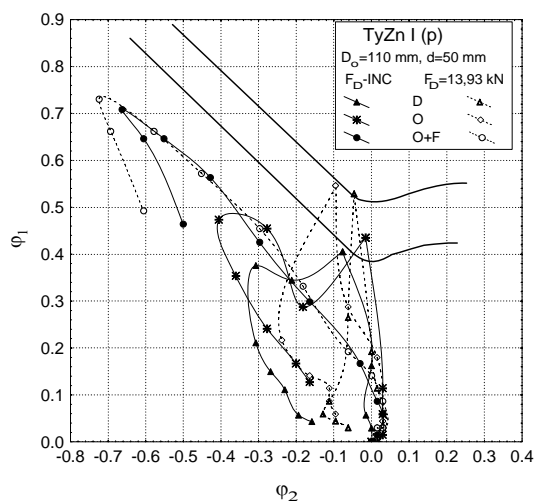
Figure 14. Strain distribution in plane at increasing VBF
