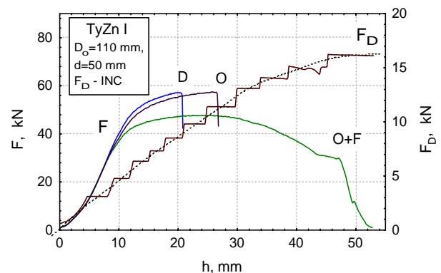
Figure 13. Dependence of drawing force and increasing blank holding force on travel
