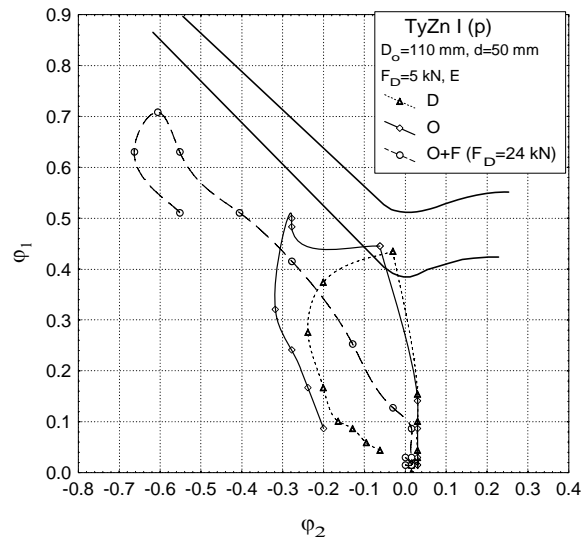
Figure 12. Strain distributions in sheet metal plane (CBF-E)
