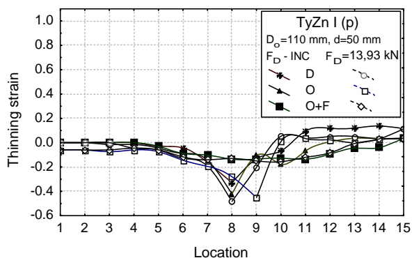
Figure 15. Thinning distribution at increasing VBF
