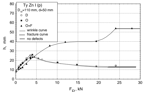
Figure 7. Dependence of drawing depth on blank holding force (a)
