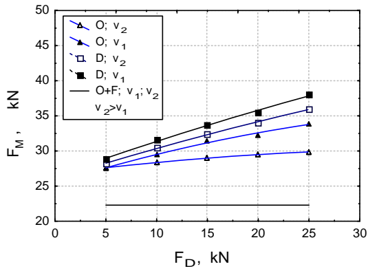
Figure 5. Dependence of maximal drawing force on blank holding force (a)
