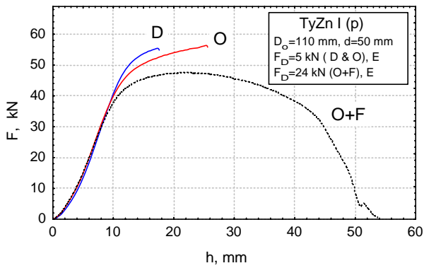
Figure 10. Drawing forces at CBF (version E)
