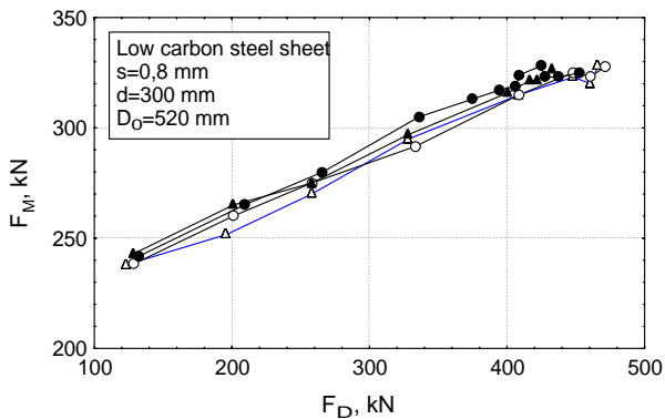
Figure 6. Dependence of maximal drawing force on blank holding force (b)
