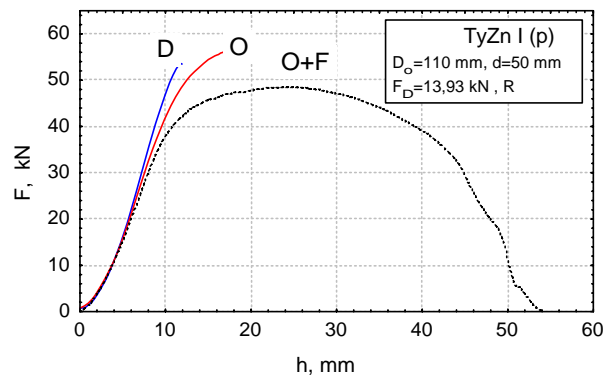
Figure 9. Drawing forces at CBF (version R)
