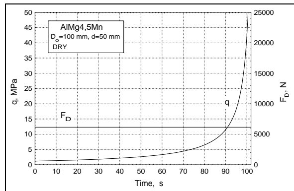
Figure 7. Constant BHF
