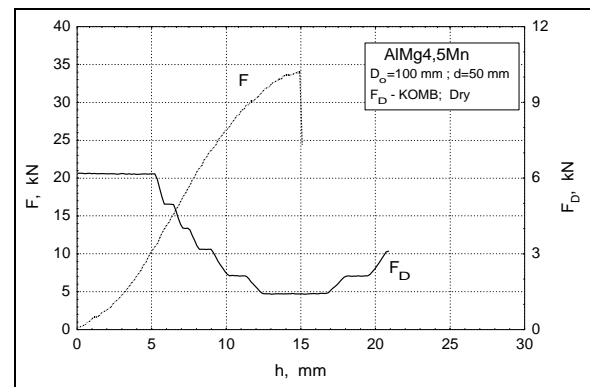
Figure 10. Drawing and BHF forces
