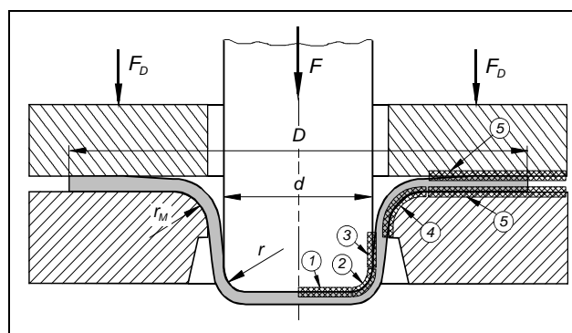
Figure 1. Friction zones in deep drawing process
