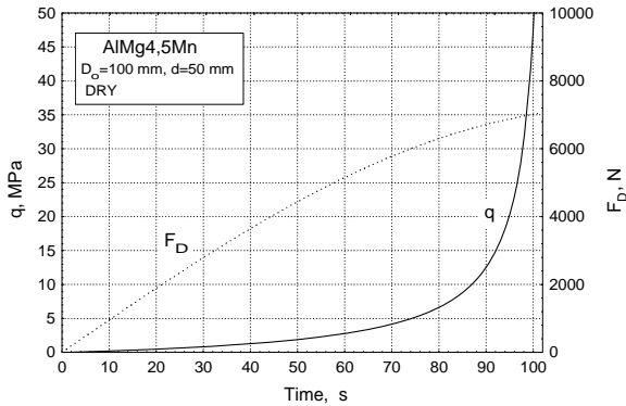
Figure 4. Increasing BHF
