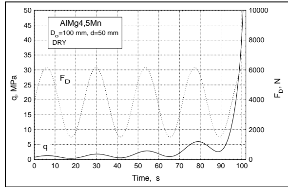
Figure 6. Pulsating VBHF
