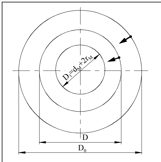
Figure .2 Flange area change durig the process
