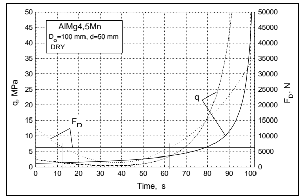
Figure 5. Combined VBHF
