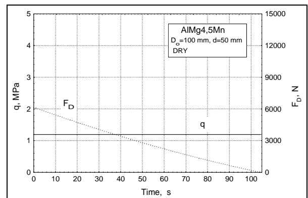
Figure 3. Decreasing BHF
