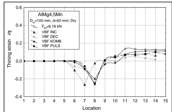
Figure 8. Distributions of thinning strain
