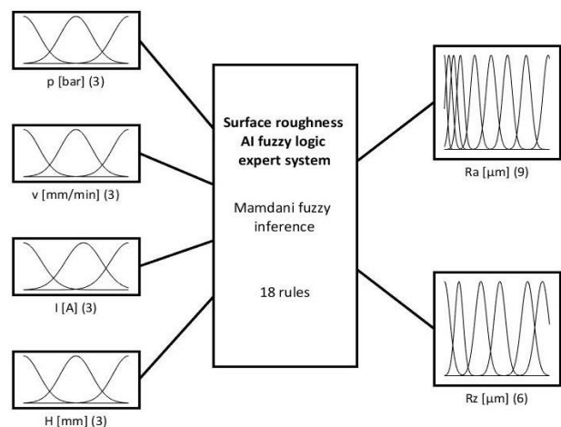
Figure 4. AI fuzzy logic system for modeling and prediction surface roughness response
