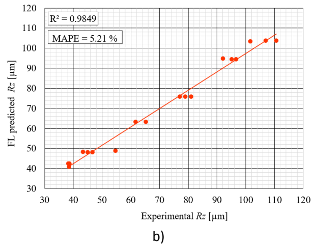
Figure 8. Comparison between FL predicted and experimental data of: a) Ra , b) Rz
