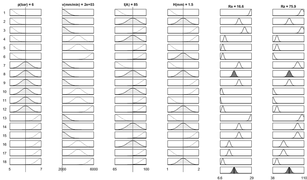
Figure 7. Base of fuzzy IF-THEN rules between inputs: p , v , l , H and outputs: Ra , Rz
