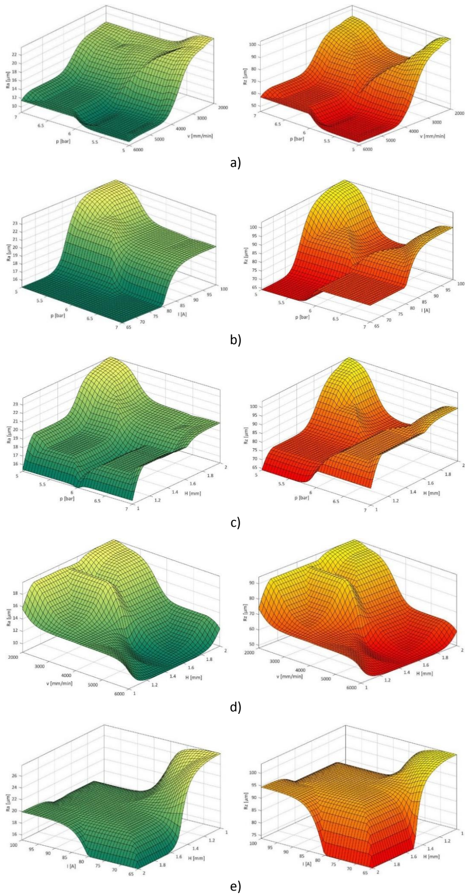
Figure 9. Process parameters effects on surface roughness Ra and Rz when constant parameters are: a) I = 100 A, H = 2 mm, b) v = 2000 mm/min, H = 2 mm, c) v = 2000 mm/min, I = 100 A, d) p = 7 bar, I = 100 A, e) p = 7 bar, v = 2000 mm/min
