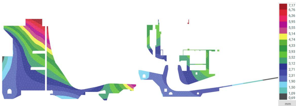
Fig. 5. Field of displacement in the direction of the Danube (mm) on pier 10 of the spillway dam and section III of the power plant
