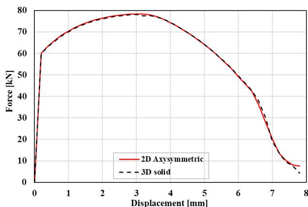
Figure 6. Force-displacement response for 3D solid FE model and 2D axisymmetric FE model.
