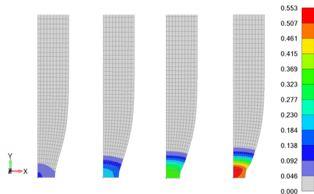
Figure 12. Damage field evolution in the last four time-steps of the simulation (50th-53rd, from left to right).
