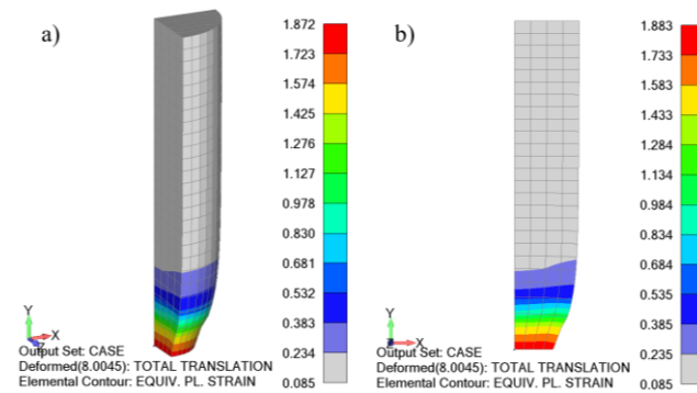
Figure 4. Equivalent plastic strain field in the last (40th) time step for: a) 3D solid; and b) 2D axisymmetric FE model, /28/.
