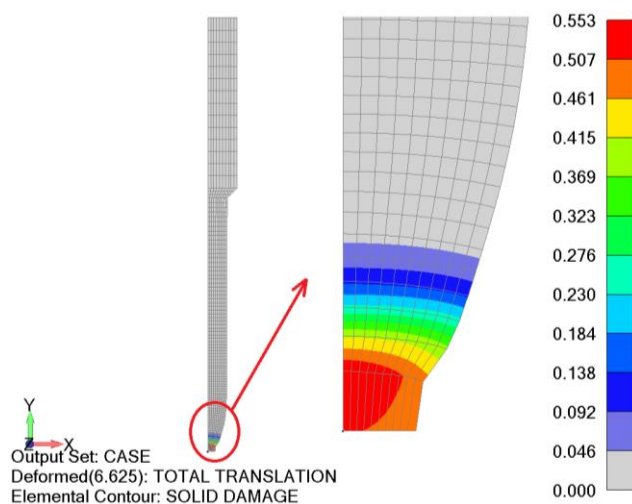
Figure 10. Damage field in last converged (53rd) time step.
