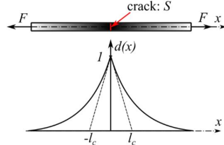
Figure 1. A bar loaded by forces F on both sides with a crack surface S in the middle: damage phase field for diffusive crack topology /5/.
