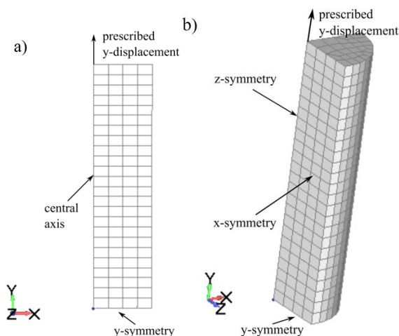
Figure 1. Boundary and loading conditions: a) 2D axisymmetric FE model; b) 3D solid FE model /28/.
