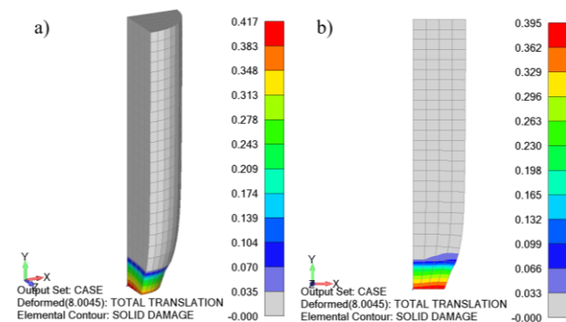
Figure 3. Damage field in the last (40th) time step for: a) 3D solid; and b) 2D axisymmetric FE model, /28/.
