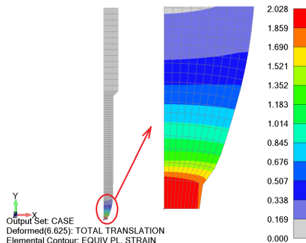
Figure 11. Equivalent plastic strain field in last converged (53rd) time step.
