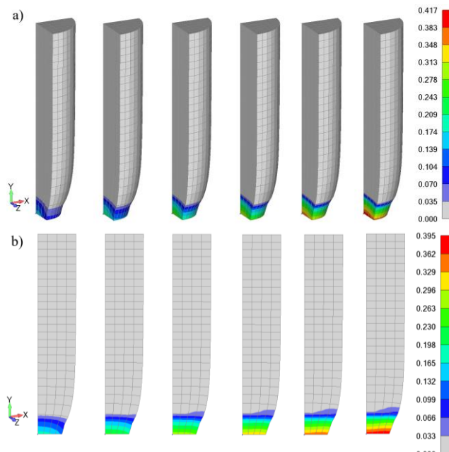
Figure 5. Damage field evolution in the last six time steps of the simulation (35th-40th, from left to right) for: a) 3D FE model; and b) 2D axisymmetric FE model, /28/.
