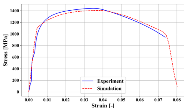
Figure 13. Comparison of stress-strain curve for experiment and simulation.
