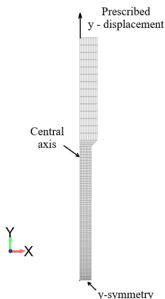
Figure 9. 2D axisymmetric FE specimen model with boundary conditions.
