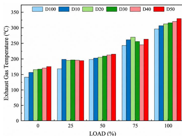
Figure 1 Variation in exhaust gas temperature as a function of engine load for diesel fuel and different biodiesel blends (Karrar & Hyder, 2026)
