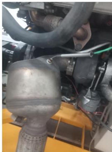
Figure 4 Thermocouple for exhaust gas temperature measurement
