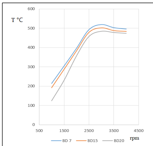
Figure 7 Exhaust gas temperature at full engine load (100% load)
