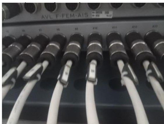
Figure 5 Connection of thermocouples to the F-FEM-AIS module
