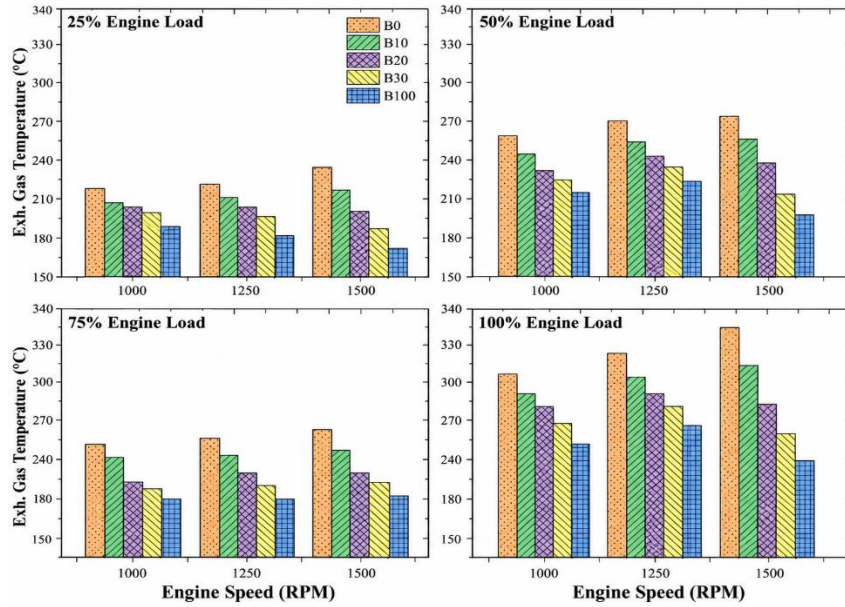
Figure 2 Variation in exhaust gas temperature (Karabulut et al. 2024)
