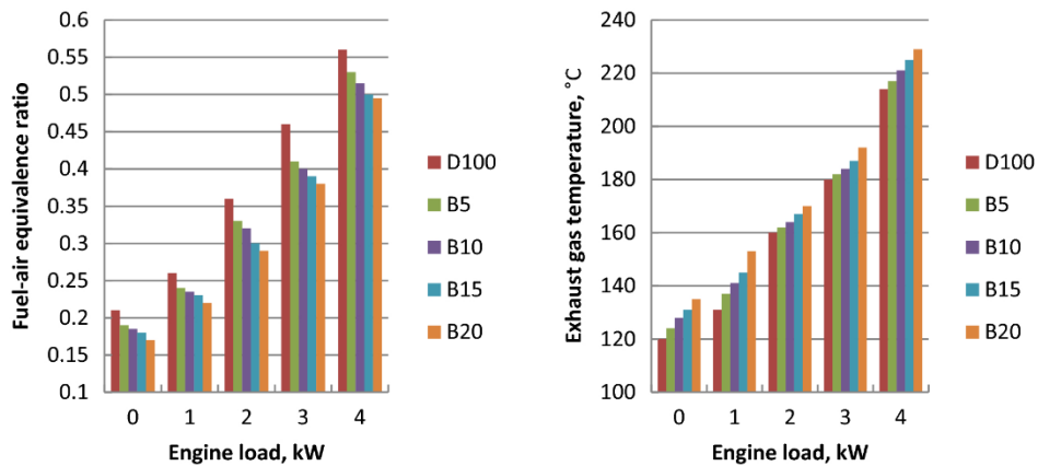
Figure 3 Variation of the fuel–air equivalence ratio and exhaust gas temperature (Text) as a function of engine load (El-Shafay et al. 2022)
