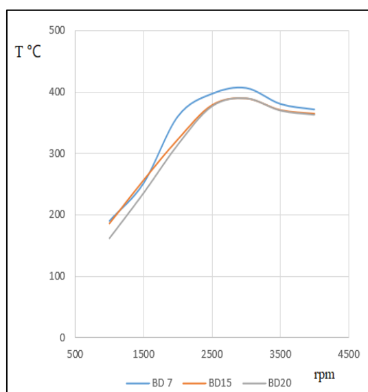
Figure 6 Exhaust gas temperature at a partial engine load of 50%
