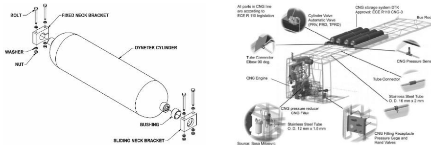
Figure 5 Cylinder Neck Mount Assembly and Installation of the Cylinder Rack on the Roof of a City Bus
