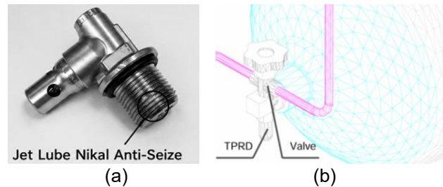
Figure 3 (a) Application of Anti-Seize Compound to the Valve Thread; (b) Typical Valve and TPRD Assembly
