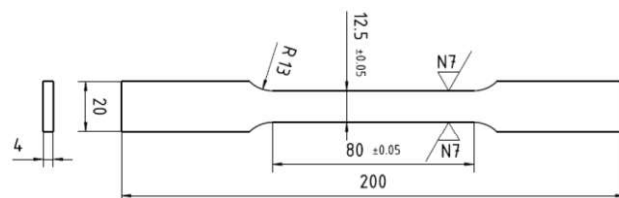
Figure 2. Drawing for samples preparation
