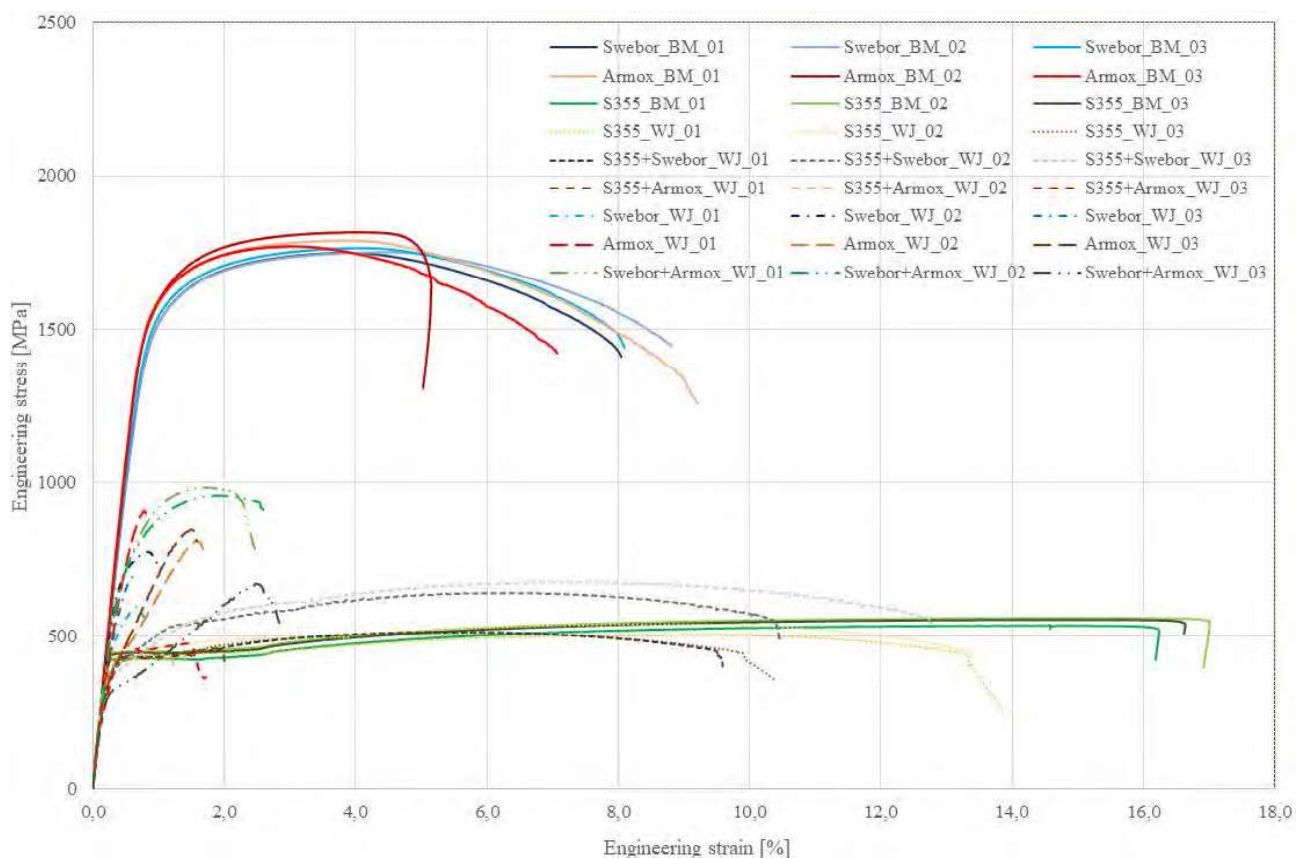
Figure 7. Stress-strain diagrams for tested specimens
