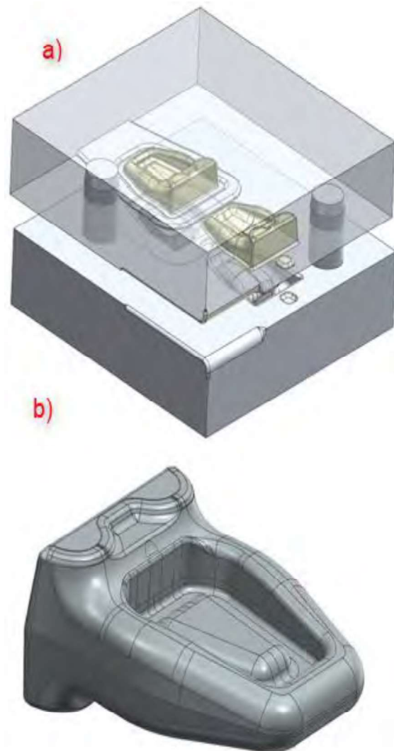
Figure 1. 3D model: a) Upper and lower die for forging; b) Forged part
