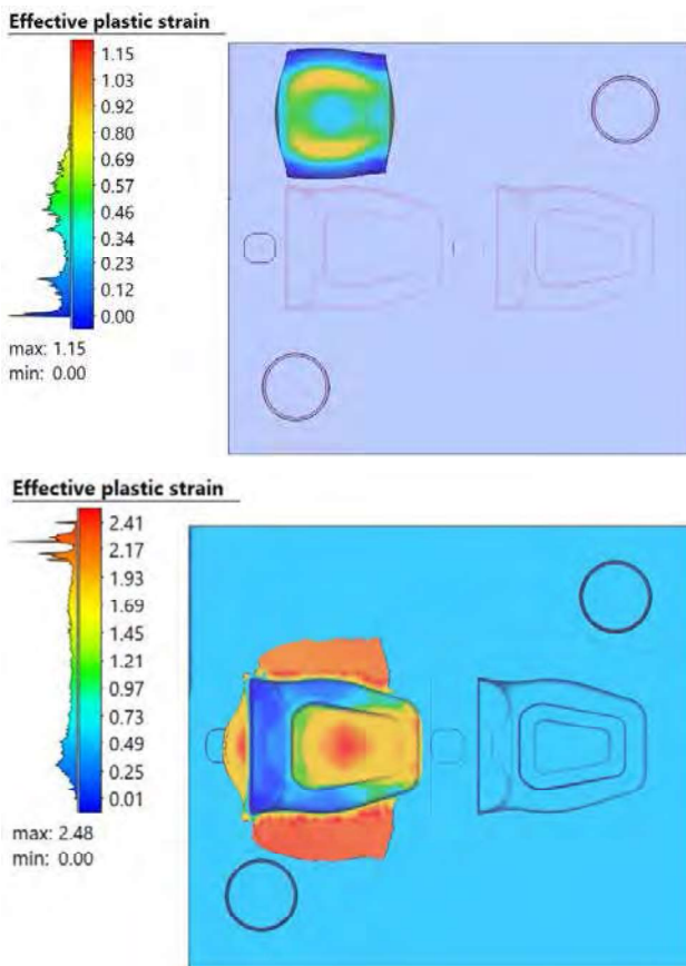
Figure 2. Upsetting and pre-forging
