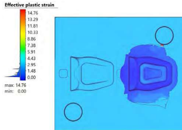
Figure 4. Value of effective plastic strain mesh 2.2 mm
