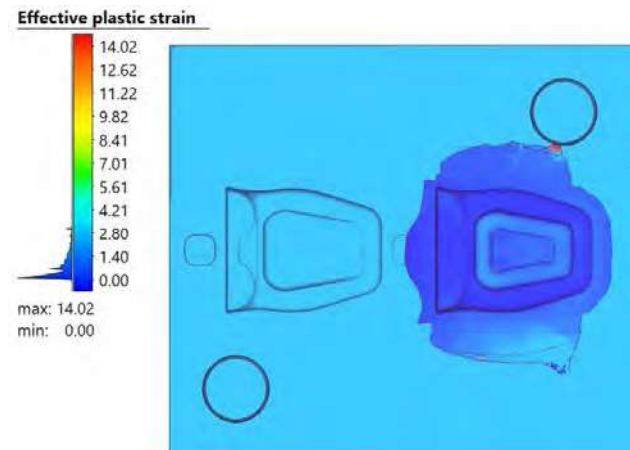
Figure 5. Value of effective plastic strain mesh 1.5 mm
