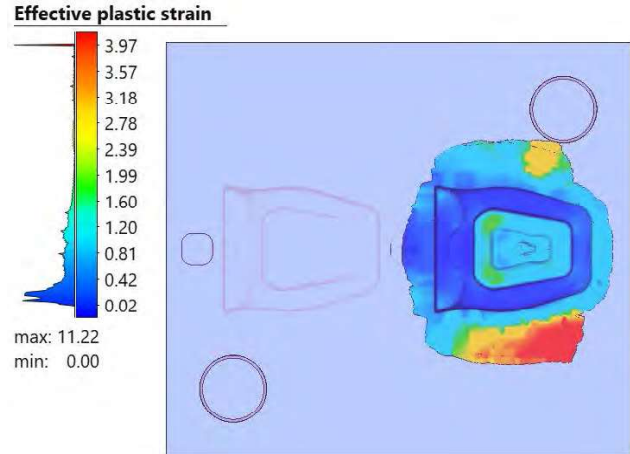
Figure 3. Value of effective plastic strain mesh 3 mm
