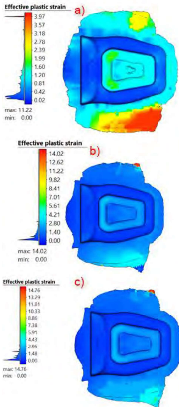
Figure 6. Forged part: a) Mesh 3.0 mm b) Mesh 2.2 mm c) Mesh 1.5 mm
