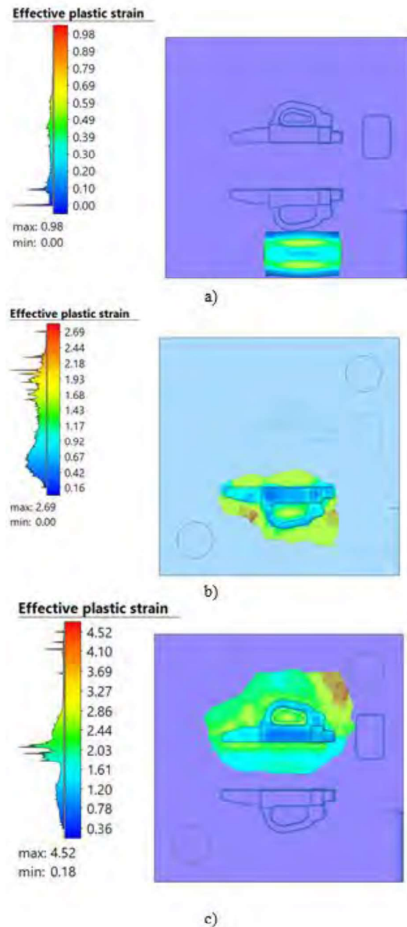
Figure 3. Value of Plastic Strain for second case: a) Upsetting; b) Pre-forging; c) Final forging
