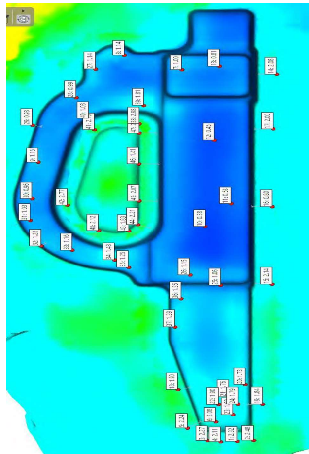
Figure 4. Plastic Strain point on forging part first case
