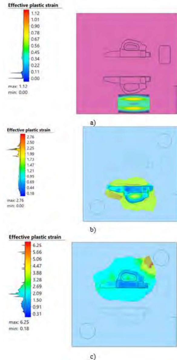
Figure 2. Value of Plastic Strain for first case: a) Upsetting; b) Pre-forging; c) Final forging
