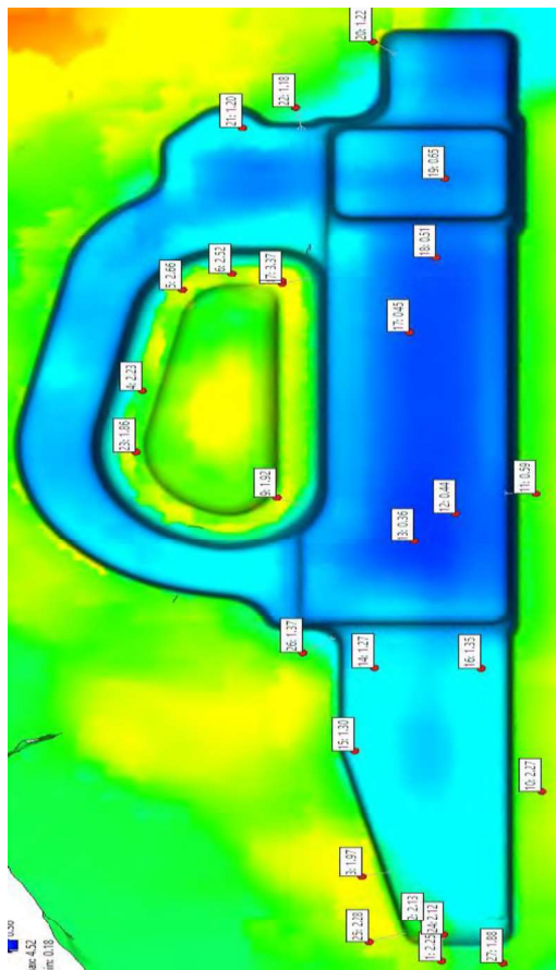
Figure 5. Plastic Strain point on forging part second case
