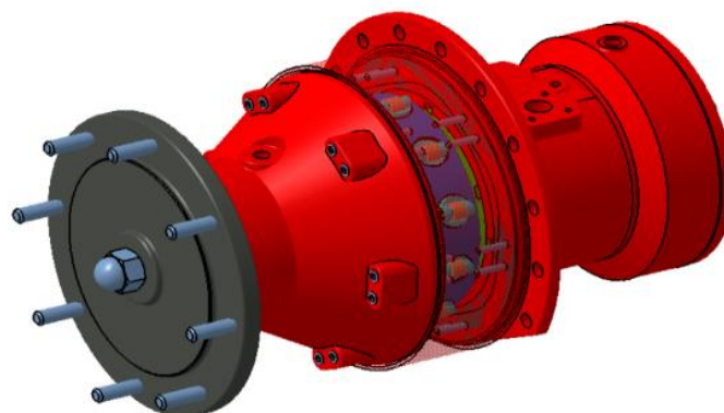
Figure 2 3D model of Radial piston hydraulic motor
