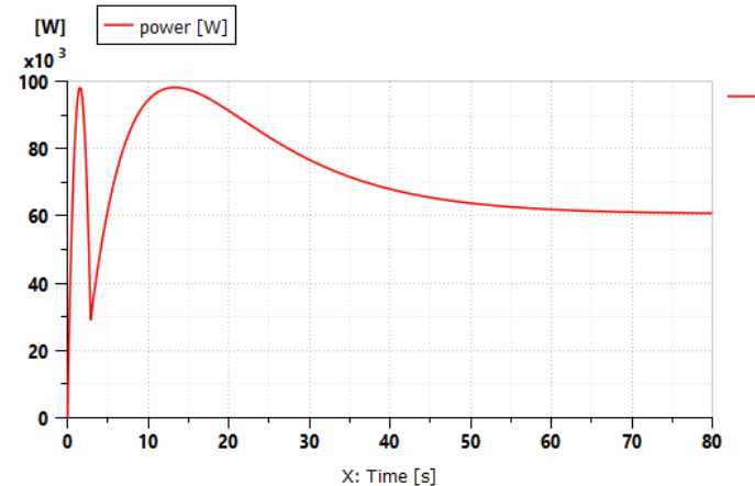
Figure 13 Simulated engine power of the minibus (Siemens Digital Industries Software, 2020)
