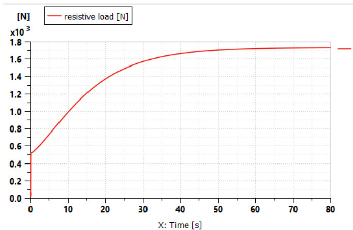
Figure 11 Simulated resistive load of the minibus (Siemens Digital Industries Software, 2020)
