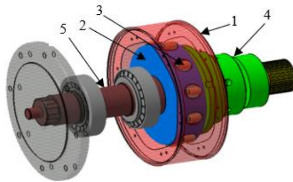
Figure 3 Key parts of radial hydraulic motor
