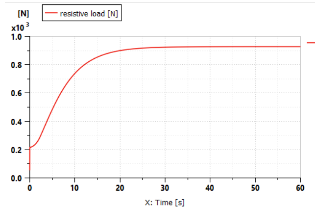
Figure 20 Simulated mini-truck resistive load under the slope of 8% (Siemens Digital Industries Software, 2020)
