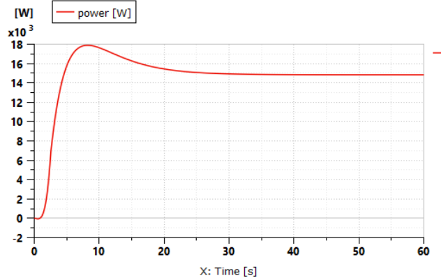
Figure 24 Simulated mini-truck axle power under the slope of 8% (Siemens Digital Industries Software, 2020)
