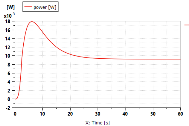
Figure 14 Simulated axle power of the mini-truck (Siemens Digital Industries Software, 2020)
