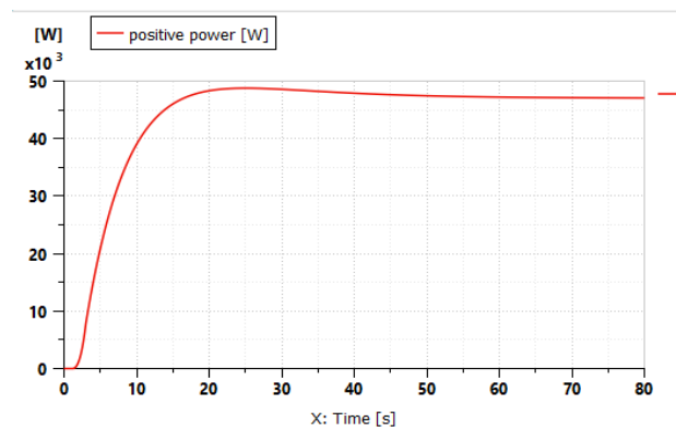
Figure 25 Simulated minibus axle power under the slope of 8% (Siemens Digital Industries Software, 2020)
