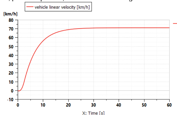
Figure 16 Diagram of simulated mini-truck velocity under the slope of 8% (Siemens Digital Industries Software, 2020)
