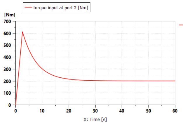
Figure 18 Diagram of simulated mini-truck axle torque under the slope of 8% (Siemens Digital Industries Software, 2020)
