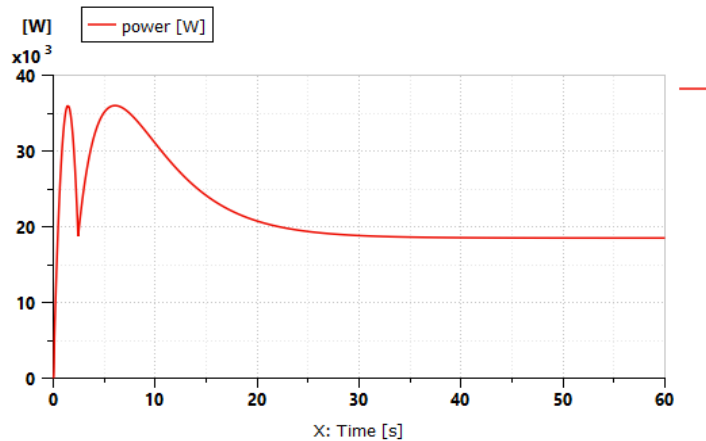
Figure 12 Simulated engine power of the mini-truck (Siemens Digital Industries Software, 2020)
