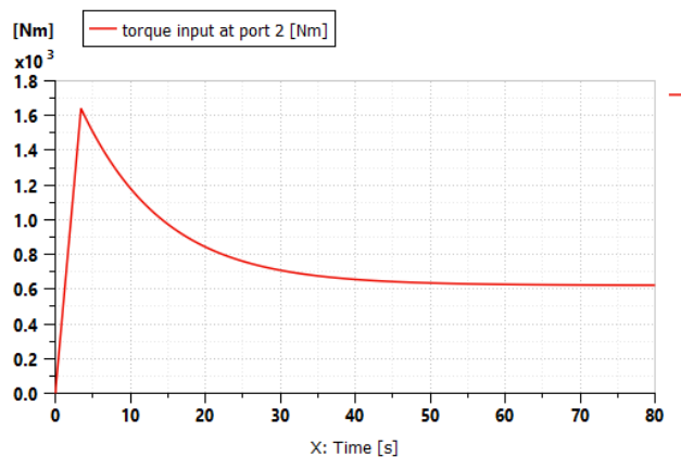
Figure 19 Diagram of simulated minibus axle torque under the slope of 8% (Siemens Digital Industries Software, 2020)
