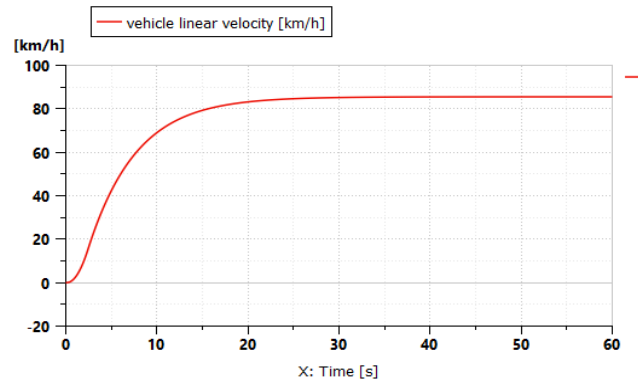
Figure 6 Diagram of simulated mini – truck velocity in 60 s operational cycle (Siemens Digital Industries Software, 2020)
