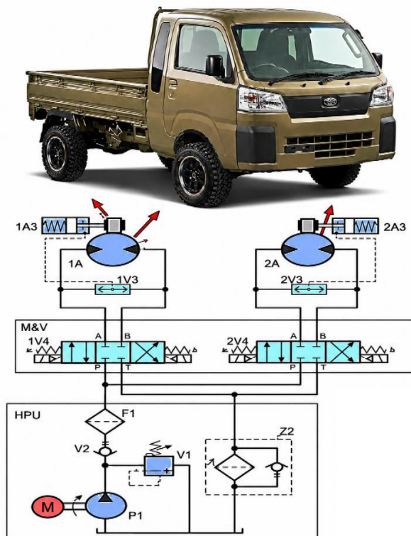
Figure 4 Schematic diagram of conventional hydraulic propulsion system of the mini – truck
