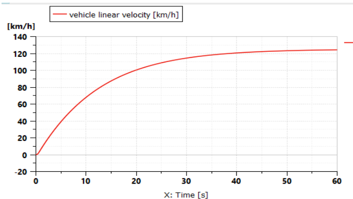
Figure 7 Diagram of simulated minibus velocity in 60s operational cycle (Siemens Digital Industries Software, 2020)
