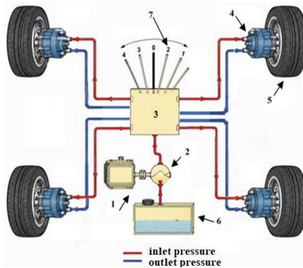
Figure 1 Schematic representation of the hydraulic drive system (Sonale, 2024)
