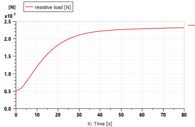
Figure 21 Simulated minibus resistive load under the slope of 8% (Siemens Digital Industries Software, 2020)
