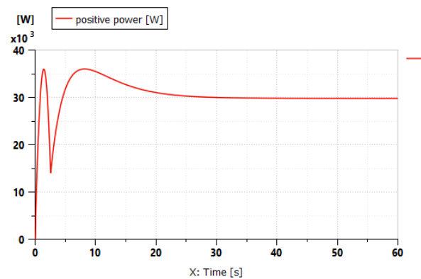
Figure 22 Simulated mini-truck engine power under the slope of 8% (Siemens Digital Industries Software, 2020)
