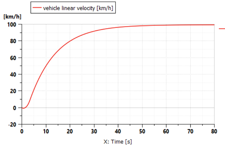
Figure 17 Diagram of simulated minibus velocity under the slope of 8% (Siemens Digital Industries Software, 2020)
