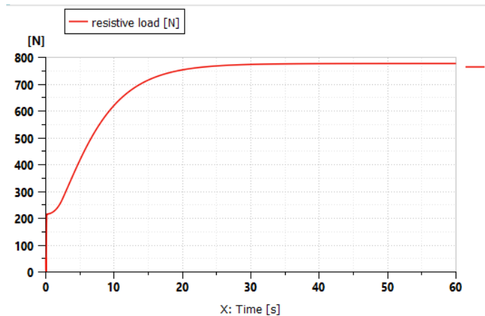
Figure 10 Simulated resistive load of the mini-truck (Siemens Digital Industries Software, 2020)
