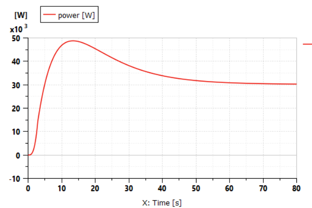
Figure 15 Simulated axle power of the minibus (Siemens Digital Industries Software, 2020)
