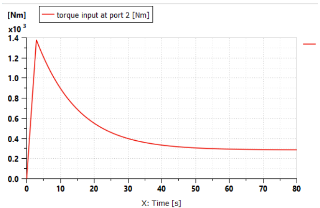
Figure 9 Simulated torque input profile at one axle of the minibus (Siemens Digital Industries Software, 2020)
