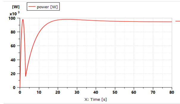
Figure 23 Simulated mini-truck engine power under the slope of 8% (Siemens Digital Industries Software, 2020)
