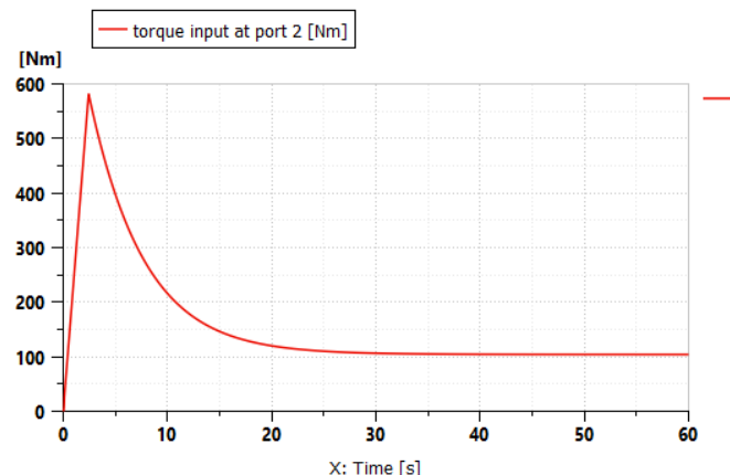
Figure 8 Simulated torque input profile at one axle of the mini – truck (Siemens Digital Industries Software, 2020)
