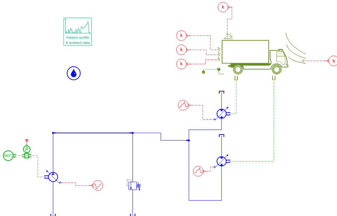
Figure 5 The lightweight transport vehicle drive diagram (Siemens Digital Industries Software, 2020)
