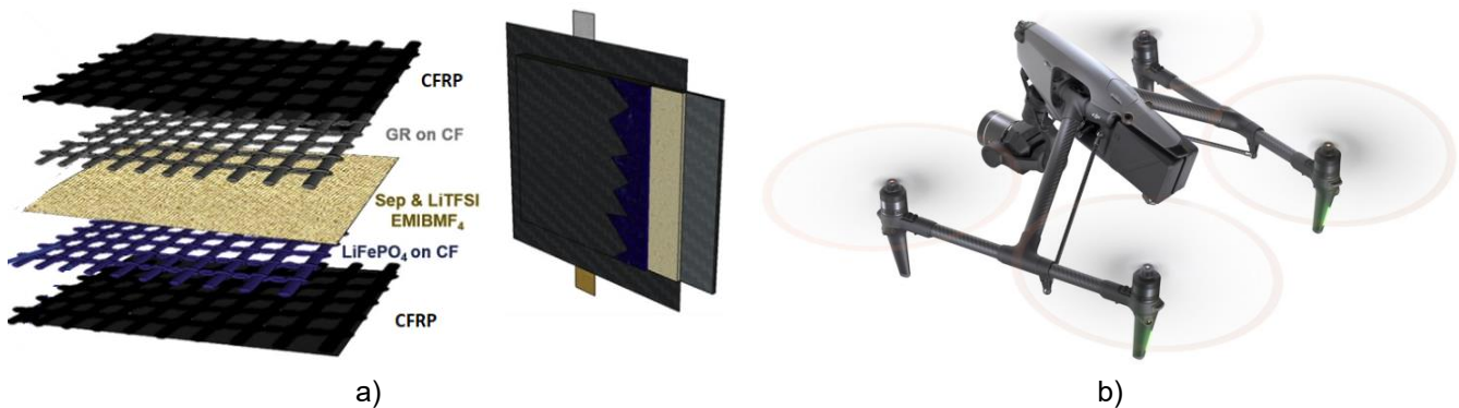
Figure 5 Applications of laminated composites in the aerospace industry: a) CFRP-reinforced lithium battery, b) Drone (DJI Inspire 3 – Master the Unseen, 2024; Moyer et al., 2020)
