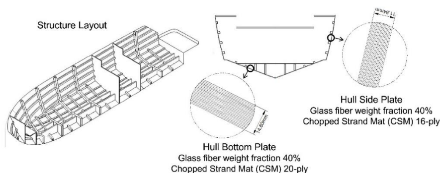
Figure 6 Hull construction and GFRP laminated panel of a composite yacht
