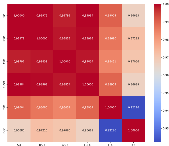
Figure 4. Correlation matrix.
