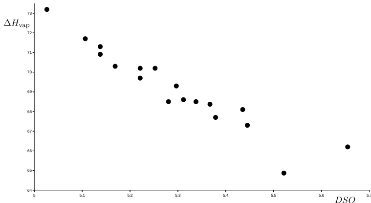
(c) Correlation between the diminished Sombor index and the heat of vaporization of octanes.
