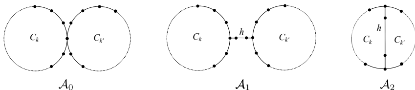
Figure 1. Bicyclic graphs without branches.
