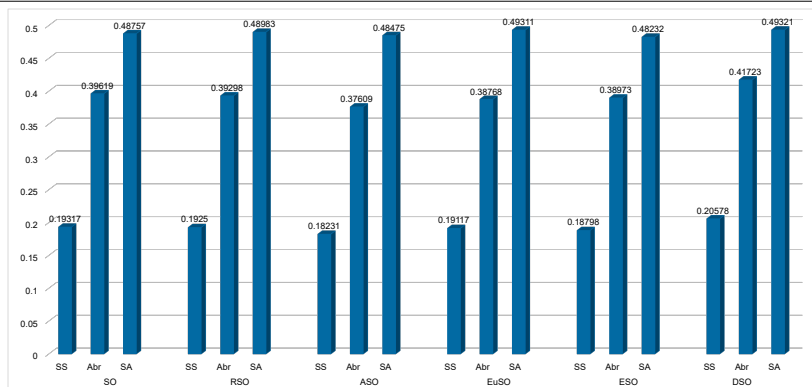
Figure 6. Structure sensitivity of the Sombor indices tested on a set of all decanes.
