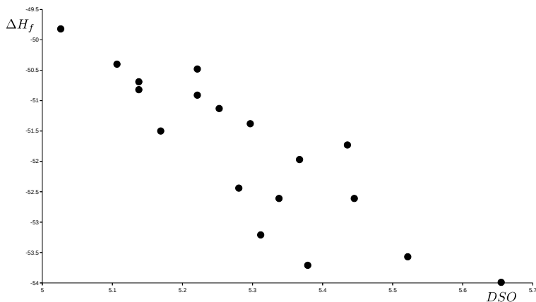
(b) Correlation between the diminished Sombor index and the heat of formation of octanes.
