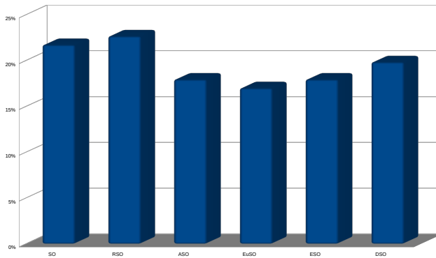
Figure 5. Degeneracy of the Sombor indices.
