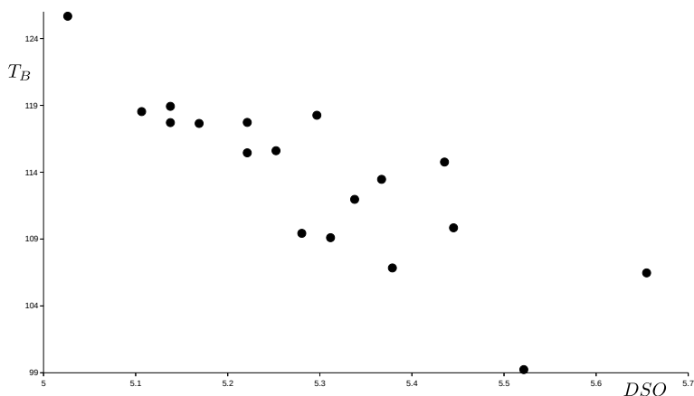
(a) Correlation between the diminished Sombor index and the boiling point of octanes.
