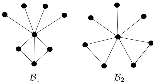
Figure 2. Bicyclic graphs considered in Theorem 15.
