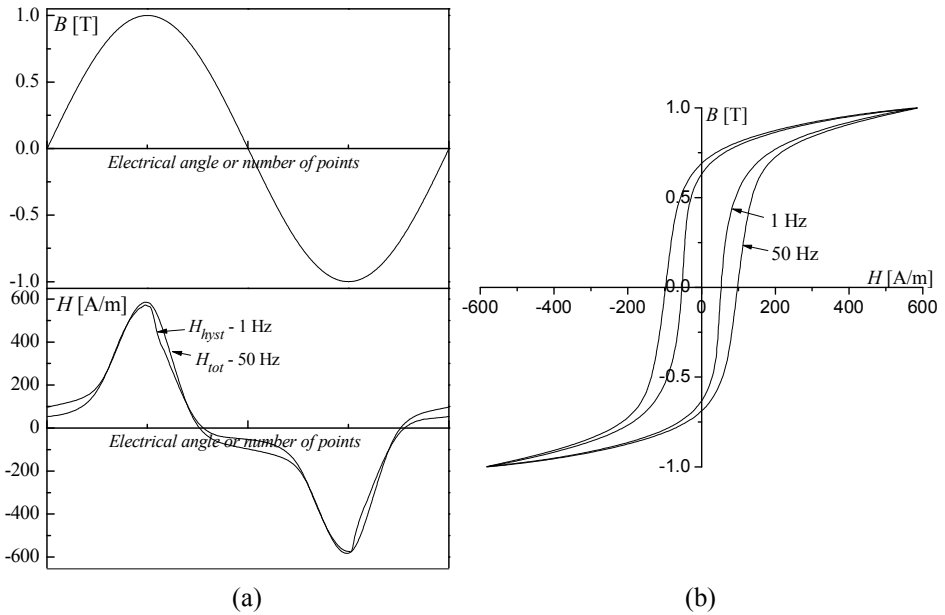
Fig. 1 – Experimental results at B_{max} = 1.0 T for 1 Hz and 50 Hz: (a) waveforms of H_{tot}(t) and H_{hyst}(t) for sinusoidal B(t) ; (b) corresponding hysteresis loops.
