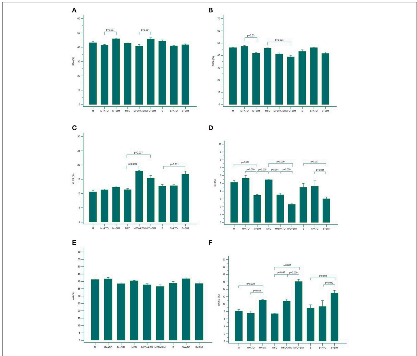
FIGURE 1 | Levels of SFA (A), PUFA (B) and MUFA (C), ω-3 PUFA (D), ω-6 PUFA (E), and ω-6/ω-3 ratio (F) in all investigated groups ( n = 8 rats per group). Results are expressed as mean ± SEM. SFA, saturated fatty acids; MUFA, monounsaturated fatty acids; PUFA, polyunsaturated fatty acids.
