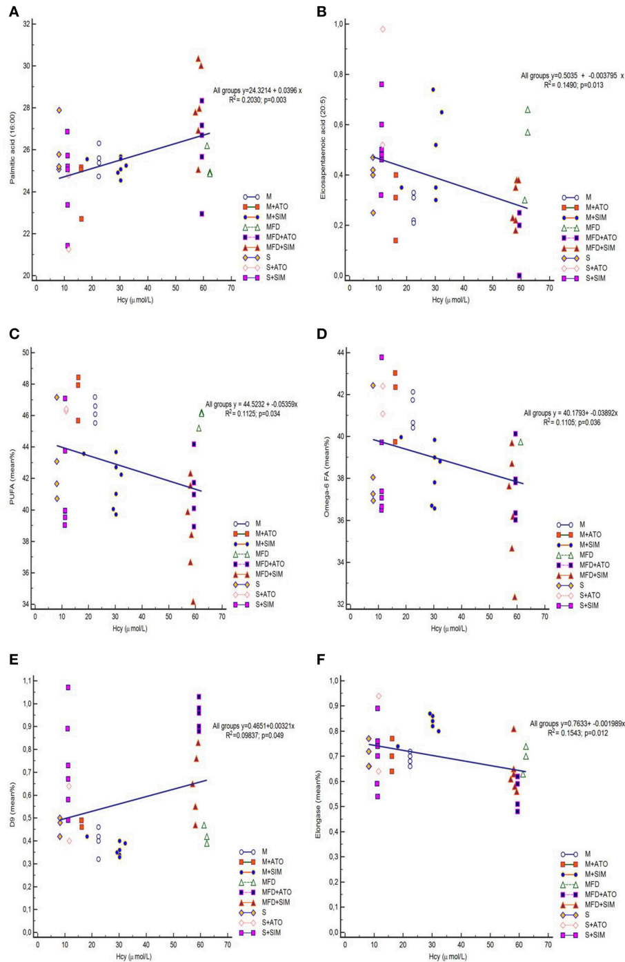
FIGURE 2 | Regression analyses. Confirmed correlation was observed between Hcy and: Palmitic acid (A), EPA (B), PUFA (C), \omega -6 PUFA (D), SCD-18 index (E), and Elongase (F) among all groups (8 rats per group). EPA, eicosapentaenoic acid; PUFA, polyunsaturated fatty acids; SCD-18, Stearoyl-CoA desaturase (18:1/18:0).
