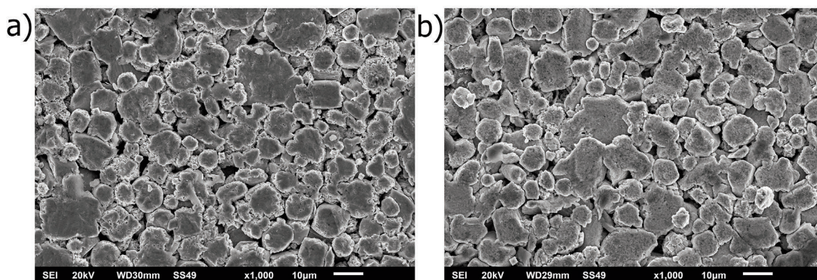
Figure 9. SEM secondary electron images of pressed NiFeWCu powder mixture milled for 60 min, thermally treated up to 693 K (a) and 873 K (b) (magnification 1000x).
