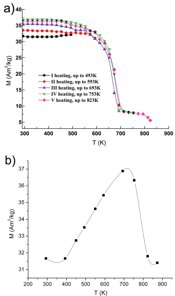
Figure 5. Temperature dependence of mass magnetization of pressed powder mechanically treated for 120 min: during successive heating (a); at room temperature as a function of the final heating temperature (b).
