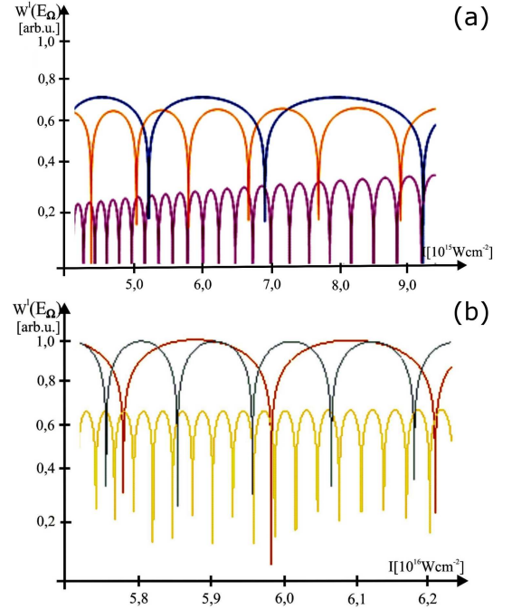
Fig. 4. Comparative review: (a) Ar atom, blue line HHG rate without any corrections of the ionization potential, magenta with spatial Gaussian pulse shape and orange with spatial Lorentzian pulse shape. Intensity varies within the range: F = 5 \times 10^{15} - 9 \times 10^{15} \text{ W cm}^{-2} , (b) K atom, red line without any correction, yellow with spatial Gaussian pulse shape and gray line with spatial Lorentzian pulse shape. Intensity varies within the range: F = 5.6 \times 10^{14} - 6.6 \times 10^{14} \text{ W cm}^{-2} . For all theoretical curves the Keldysh parameter is \gamma = 0.5 .
