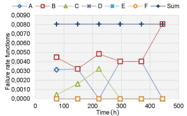
Figure 11 Rate functions per individual subsystem and total failure rate function for year 2011
