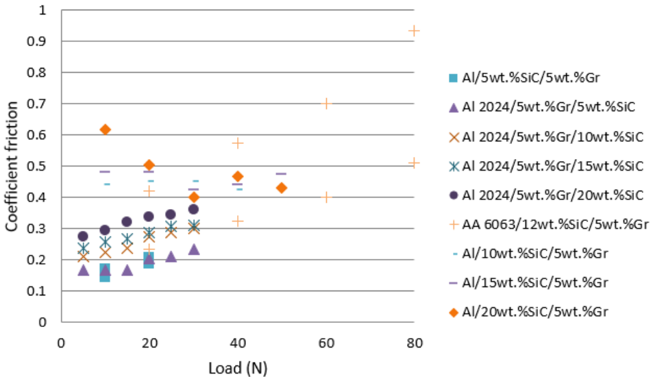
Fig. 2. The effect of load on coefficient of friction of the Al/SiC/Gr composites with different weight percentage of SiC particles and fixed 5 wt % Gr [21-24].
