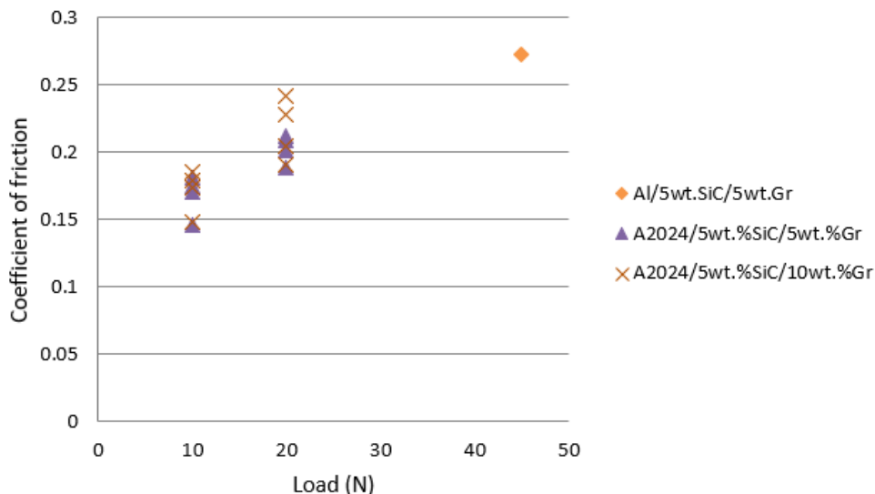
Fig. 3. The effect of load on coefficient of friction of the Al/SiC/Gr composites with different wt % of the Gr particles and fixed 5 wt % SiC [15, 25].
