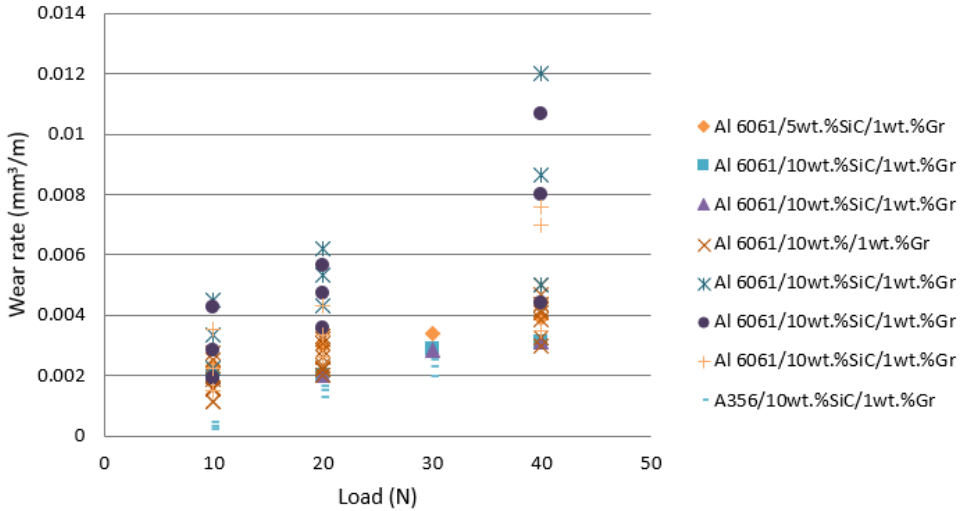
Fig. 1. The effect of load on the wear rate of the Al/SiC/Gr composites with different wt % of the SiC particles and fixed 1 wt % Gr [13, 19-20].
