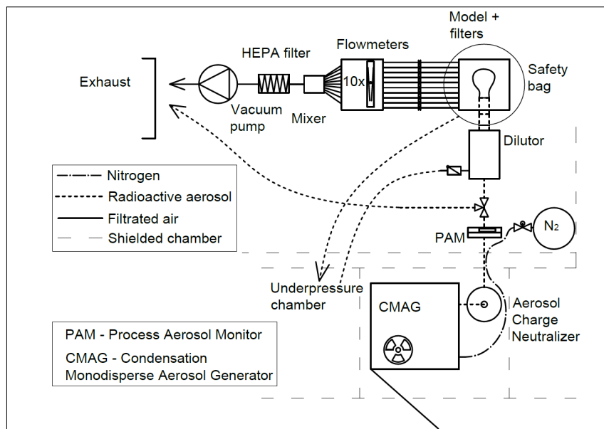
Figure 3: Schematic of the experimental set up for deposition measurements in the airways.
