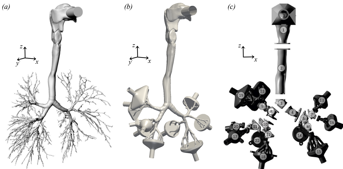
Figure 2: Geometry of the respiratory airways: (a) original realistic airway geometry; (b) geometry adopted for the benchmark case; (c) physical segmented model for deposition measurements.
