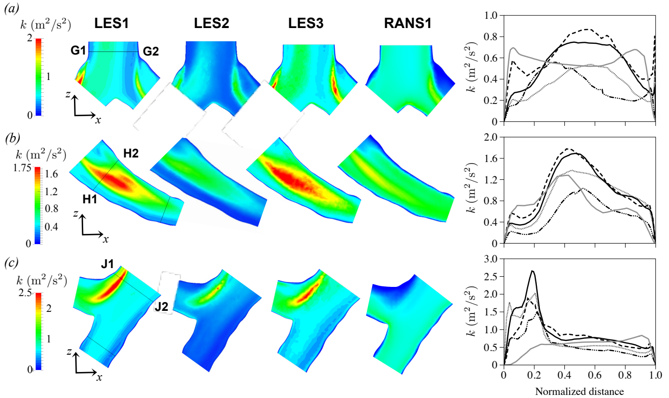
Figure 8: Contours and profiles of mean turbulent kinetic energy in (a) the carina; (b) the left main bronchus; and (c) the right main bronchus. — LES1, ..... LES1c, - - - - LES2, - - - - LES3, — RANS1.
