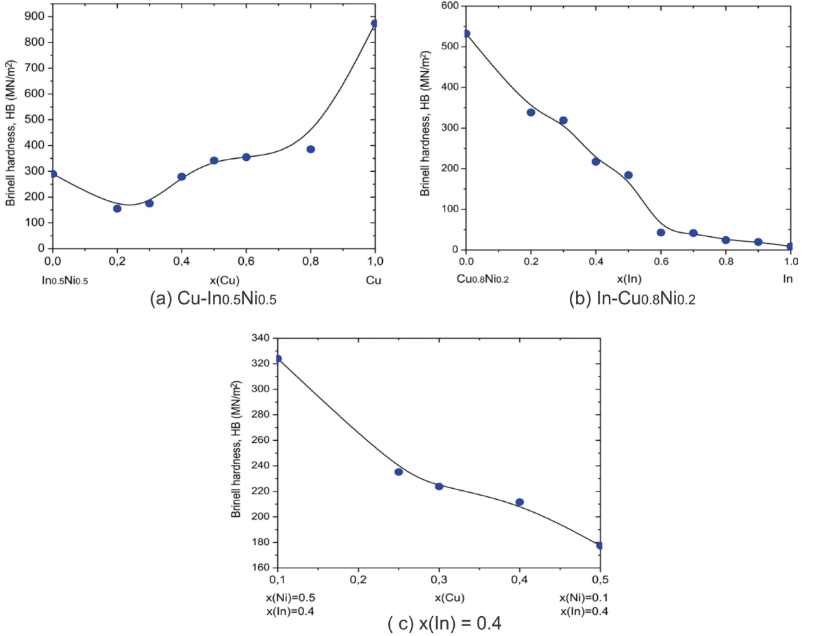
Figure 4. Measured values of Brinell hardness of the alloys from the three studied vertical sections: a) Cu-In 0.5 Ni 0.5 , b) In-Cu 0.8 Ni 0.2 and c) x(In)=0.4
