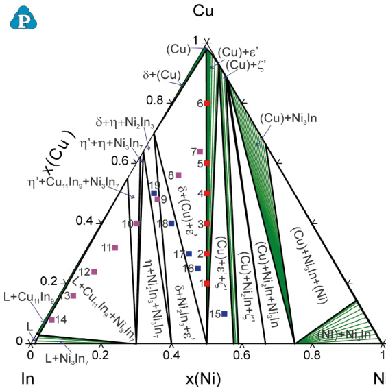
Figure 1. Predicted isothermal section of the ternary Cu-In-Ni system at 300 °C with marked compositions of the studied samples
