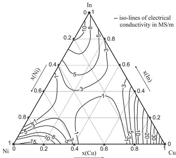
Figure 7. Iso-lines of electrical conductivity of Cu-In-Ni ternary system.
