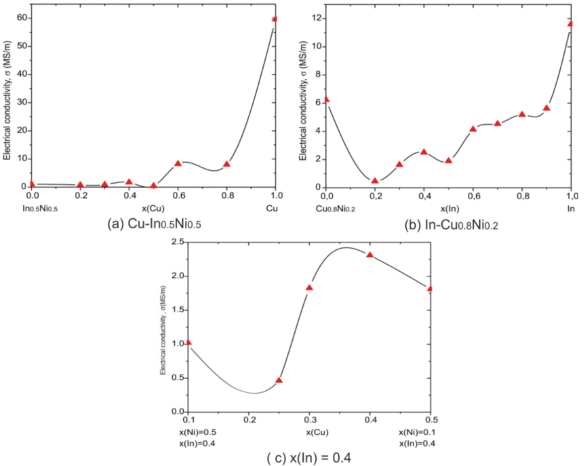
Figure 6. Experimentally determined electrical conductivity of alloys from the three studied vertical sections: a) \text{Cu-In}_{0.5}\text{Ni}_{0.5} , b) \text{In-Cu}_{0.8}\text{Ni}_{0.2} , c) x(\text{In})=0.4
