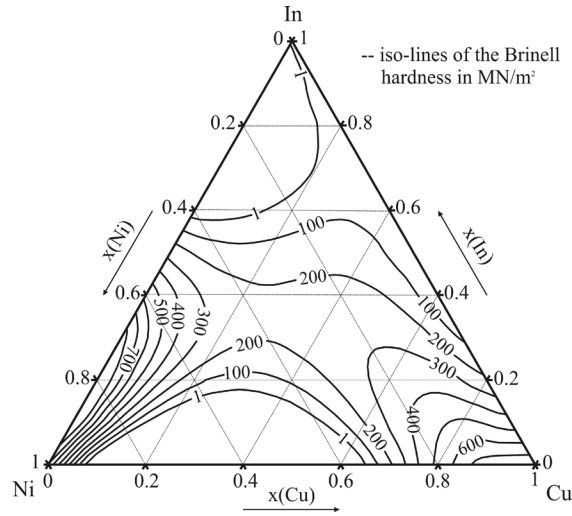
Figure 5. Iso-lines of the Brinell hardness of Cu-In-Ni ternary system.
