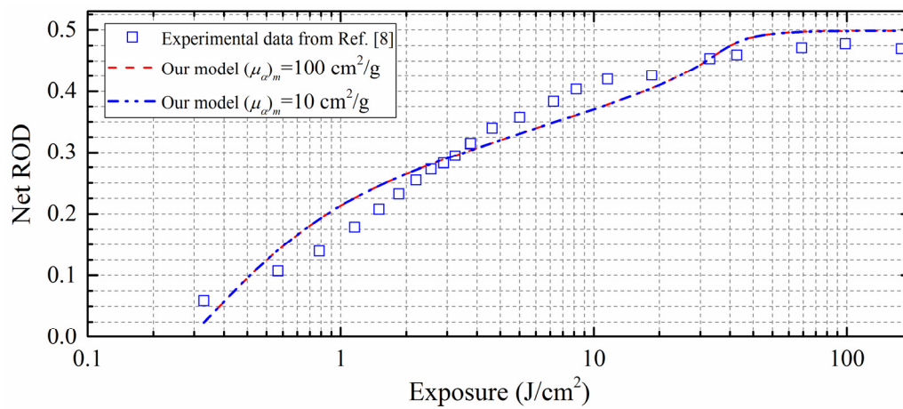
Figure 9. Comparisons among Net ROD values (obtained experimentally by Chun et al. [8] and from theoretical predictions with two different mass energy-absorption coefficients, (\mu_{\alpha})_m ) versus UV-light exposures. (The error bars for the experimental data are smaller than the symbols.)
