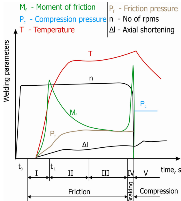
Figure 3. Dependence of friction welding parameters of welding process phase
