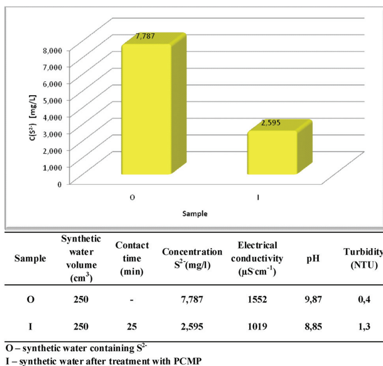
Fig. 5. Physicochemical parameters of synthetic water containing \text{S}^{2-} before and after the treatment with PCMP.
