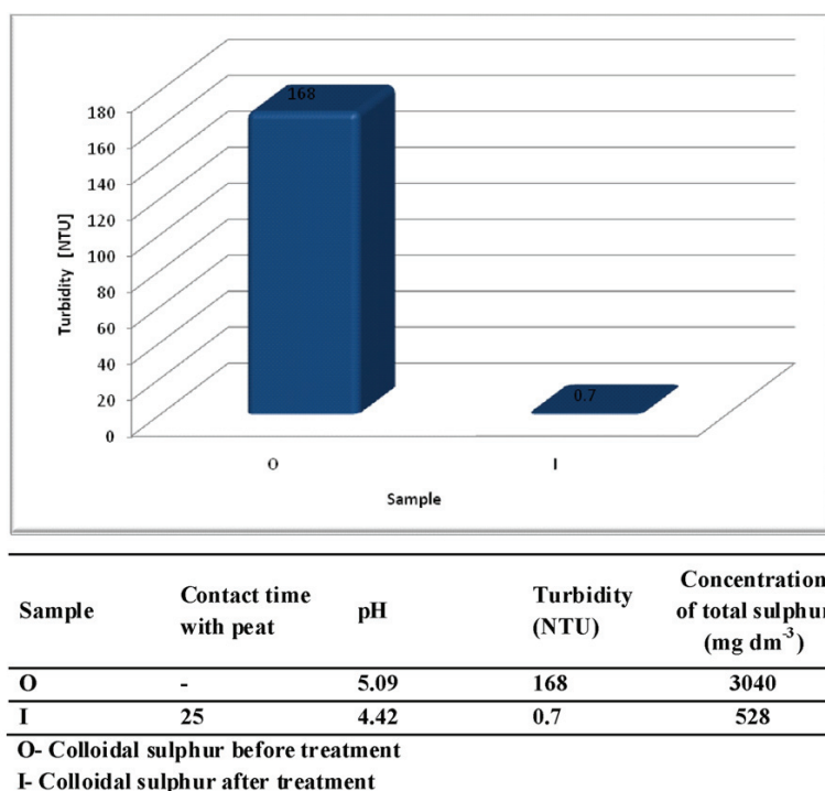
Fig. 6. Physicochemical parameters of synthetic water containing colloidal sulphur before and after the treatment with PCMP.
