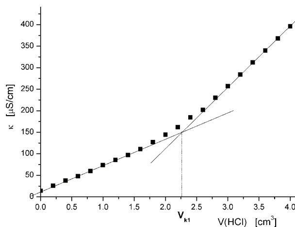
Figure 3. Conductometric titration of a suspension containing 4 \text{ g/dm}^3 PCMP with 0.025 \text{ M HCl} at 20^\circ \text{C} .
